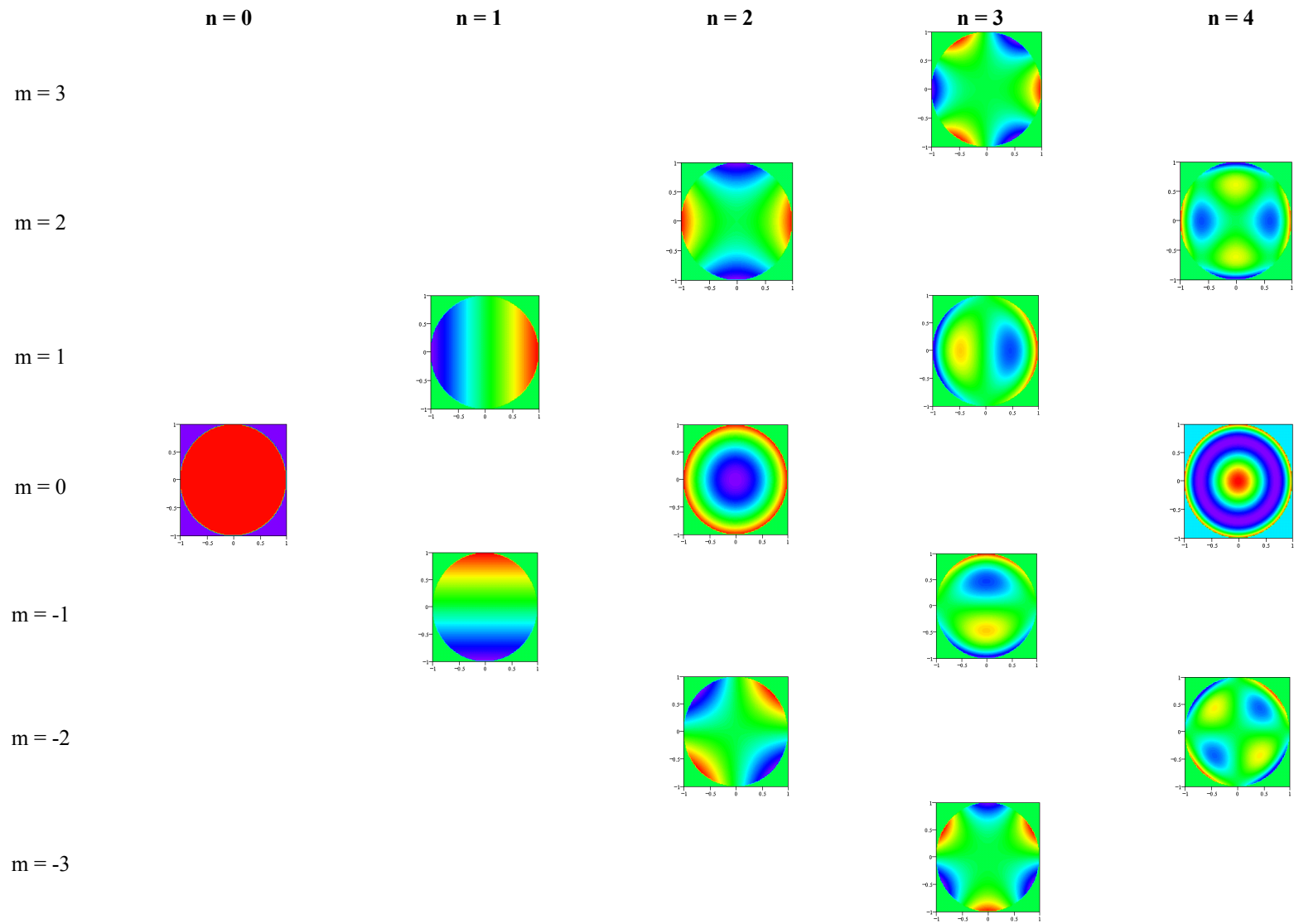
Zernike-Polynome
