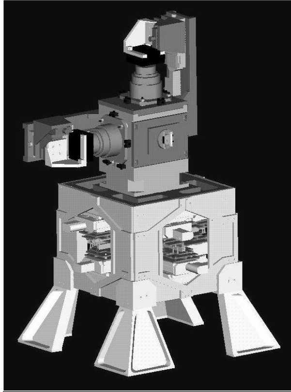
Figure 3. Mid-High Layer Wavefront Sensor (MHWS). 8 star enlarger can pick up a natural guide star (NGS) out of the center 2' FoV. The light is optically co-added on the detector. De-rotation is done with a K-mirror in the F/20 camera which is feeding the sensor with light. The light is split between mid and high layer.
