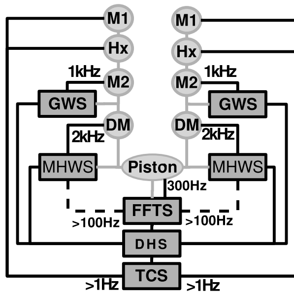
Figure 5. Extended control approach. A data handling system (DHS) is implemented to improve the performance. It will mediate through gain filtering and off loading between the single loops and the telescope control system (TCS).
