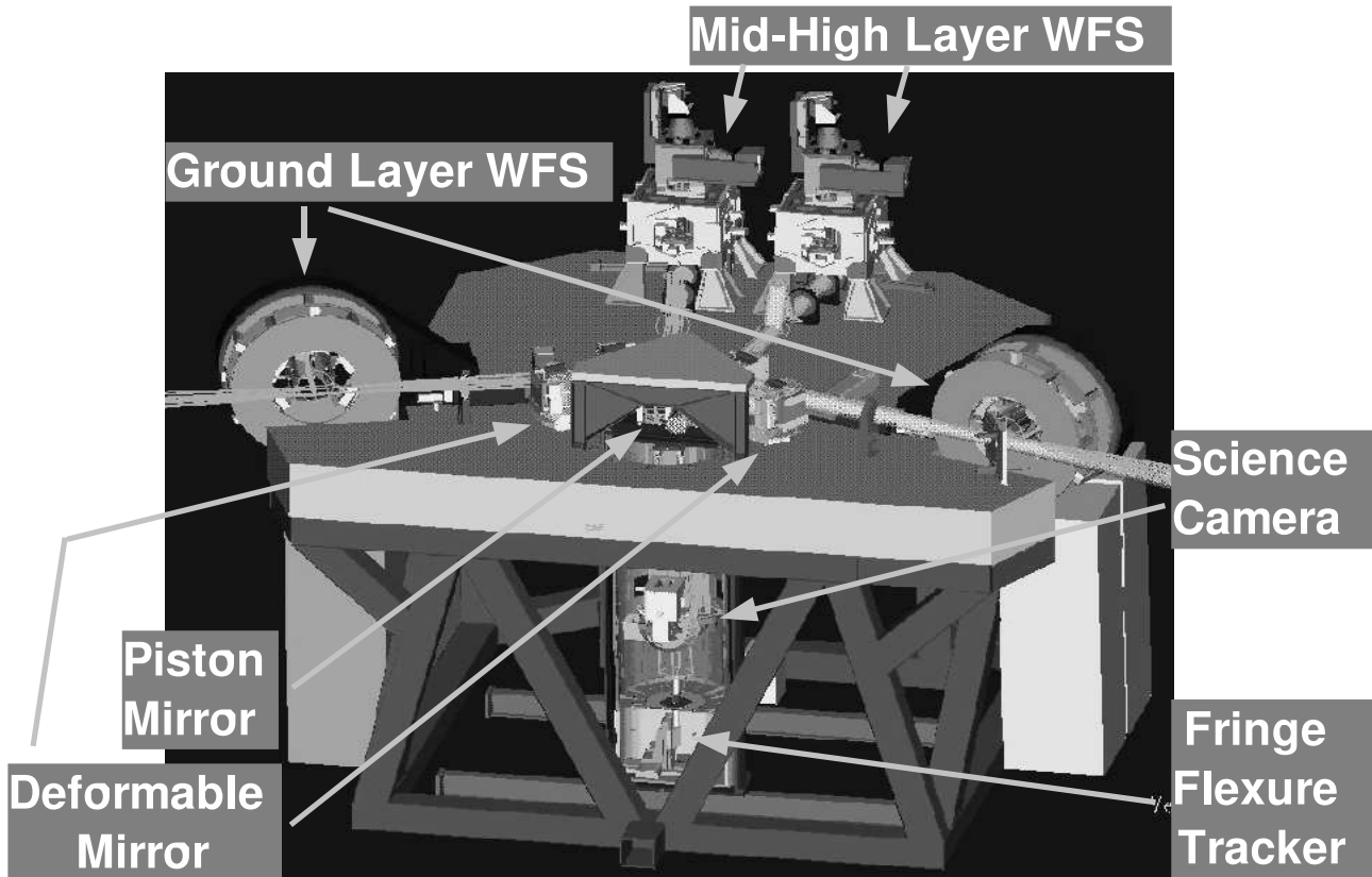
Figure 1. Overview of LINC-NIRVANA. All the major components are named. The overall dimensions of the instrument is about 3.5m x 6m x 2.5m (D x W x H).
