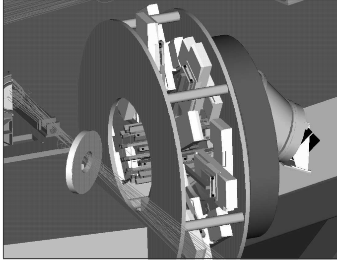
Figure 2. Ground Layer Wavefront Sensor (GWS). 12 star enlargers can pick up one guide star each out of the annular field. The light is optically co-added on the detector AT the back of the sensor. The full unit is de-rotated with a bearing.
