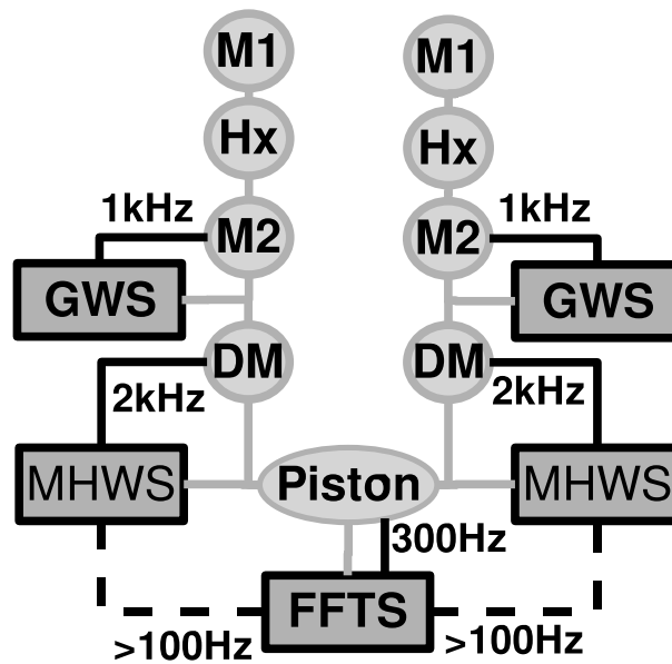
Figure 4. A simple control approach with loops in a cascade. The GWS does reduce the wavefront distortion with the adaptive secondary after that, optically decoupled, the MHWS does further wavefront improvement. The optical path difference corrected by the FFTS introduces piston which is not sensed with the MHWS and therefore does not affect the AO loop.
