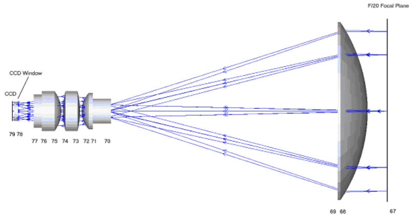
Figure 2. Patrol Camera optical layout. The optical surface numbers are referred in the text.
