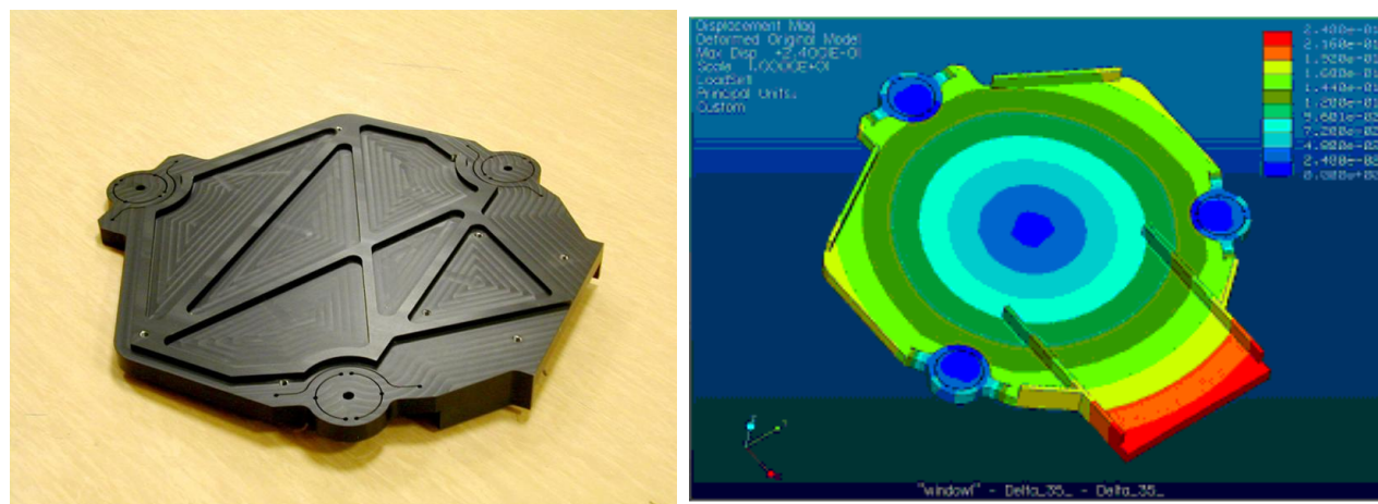
Figure 7. Left panel: Bottom view of the plate which shows the flexures and the reinforcements structures. Right panel: FEA analysis of the Flexures Plate: residual thermal variation for 35°C temperature change.
