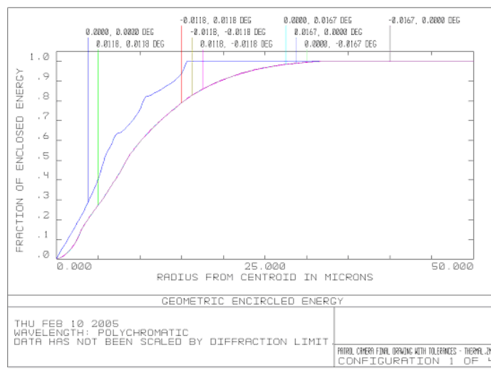
Figure 4. Encircled Energy diagram at the mean working temperature (5°C): all the light is included within a radius of \sim 30 \mu\text{m} .
