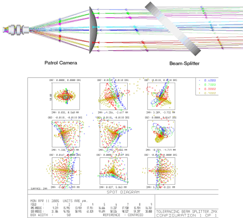
Figure 6. Top panel: Optical path through the beam-splitter. Bottom panel: The Spot Diagram (at 5°C) after introduction of the beam-splitter.
