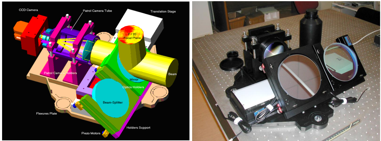
Figure 1. Left panel: Overall 3D view of the LN Patrol Camera system. Right panel: Preliminary assembly of the opto-mechanical components.
