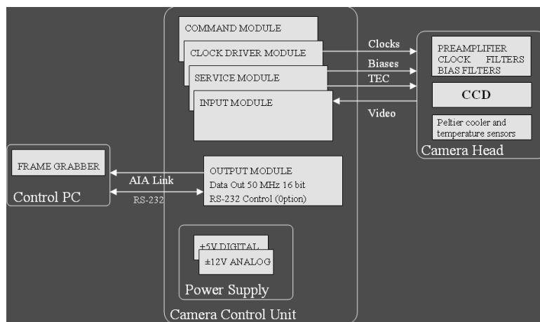
Figure 10. The Little Joe Digital Camera structure.
