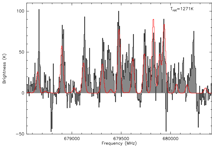
Fig. 11. Example \text{CH}_3\text{CN}(37_k - 36_k) spectrum and corresponding XCLASS two-component fit toward an arbitrary position of \text{CH}_3\text{CN} emission in the disk-like structure around source #1. The corresponding temperature is marked at the top-right.
