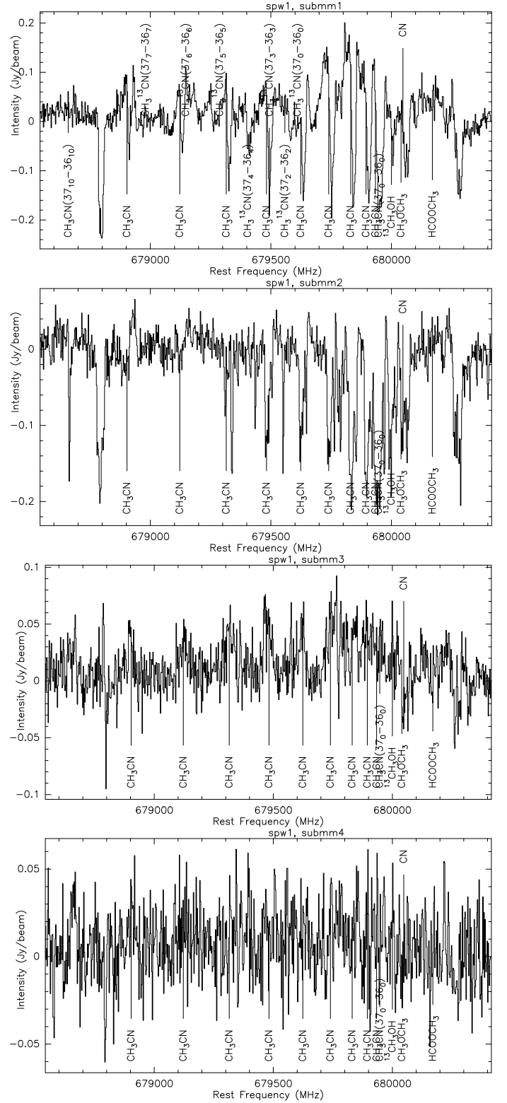
Fig. 5. Spectra extracted toward all four submm beams in spectral win spw1 averaged over 0.06'' diameter (units \text{Jy beam}^{-1} ).
