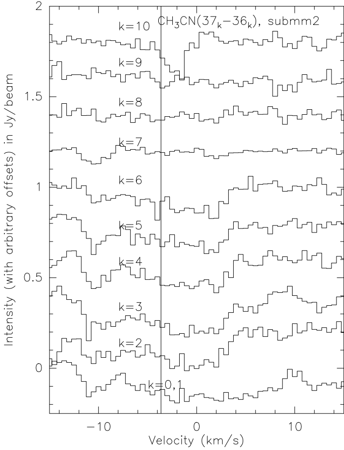
Fig. 7. \text{CH}_3\text{CN}(37_k - 36_k) spectra extracted toward the submm continuum position #2 from all k -components. The approximate v_{1sr} is marked by a vertical line, and the spectra are shifted in the y -axis for clarity.
