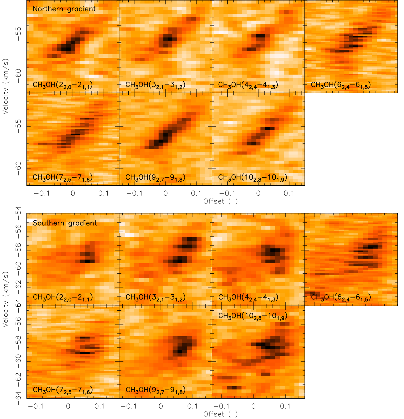
Fig. 8. Position-velocity diagrams for the different CH 3 OH lines as indicated in each panel. The top seven panels belong to the northern cut and the bottom seven panels to the southern cut shown in Fig. 7. All cuts are performed for the robust weighting 0 case.
