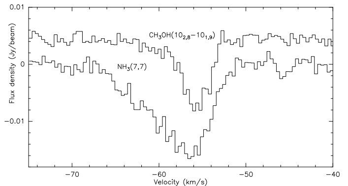
Fig. 9. Example absorption spectra of NH 3 (7,7) and CH 3 OH(10 2,8 – 10 1,9 ) taken toward the northern cm continuum peak position. The CH 3 OH spectrum is shifted slightly to positive flux density values for better presentation.
