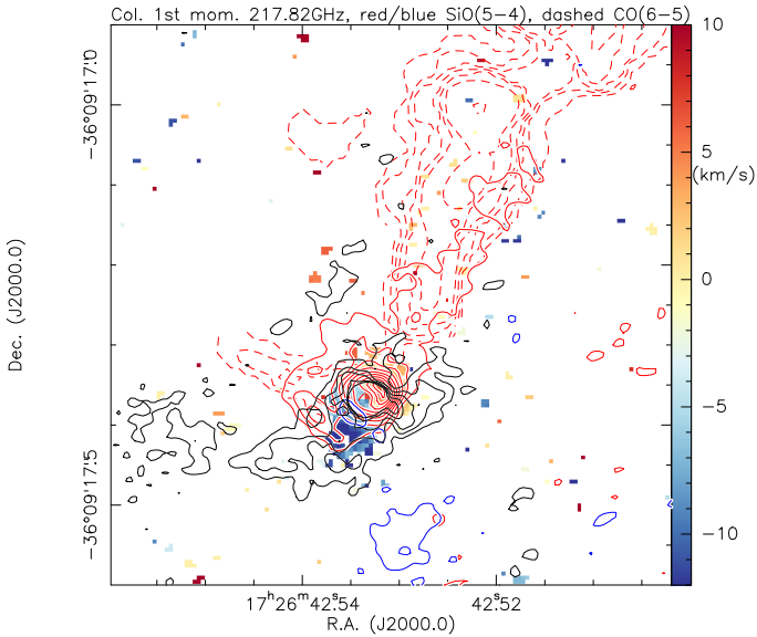
Fig. 6. Color-scale first moment map (intensity-weighted peak velocities) for mm1 from the line at 217.82 GHz. The blue and red solid contours present the blue- and redshifted SiO(5–4) emission integrated between [-22, -14] and [0, 24] \text{km s}^{-1} , respectively. The red dashed contours show the red-shifted CO(6–5) emission from Beuther et al. (2017b) . Blue-shifted CO(6–5) can not be properly imaged in that dataset, most likely because of missing short spacings. The black contours show the lower level 1.3 mm continuum data from the 4\sigma levels of 0.2 to 1.0 \text{mJy beam}^{-1} in 4\sigma steps.
