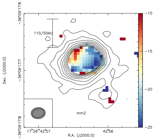
Fig. 9. Color-scale first moment map (intensity-weighted peak velocities) from the line at 231.896 GHz for the source mm2. The contours are the 1.3 mm continuum data in 4\sigma level of 0.2 \text{ mJy beam}^{-1} up to a 3 \text{ mJy beam}^{-1} level (to avoid too many contours in the center). A scale-bar and the resolution elements of the line (gray) and continuum are shown as well.
