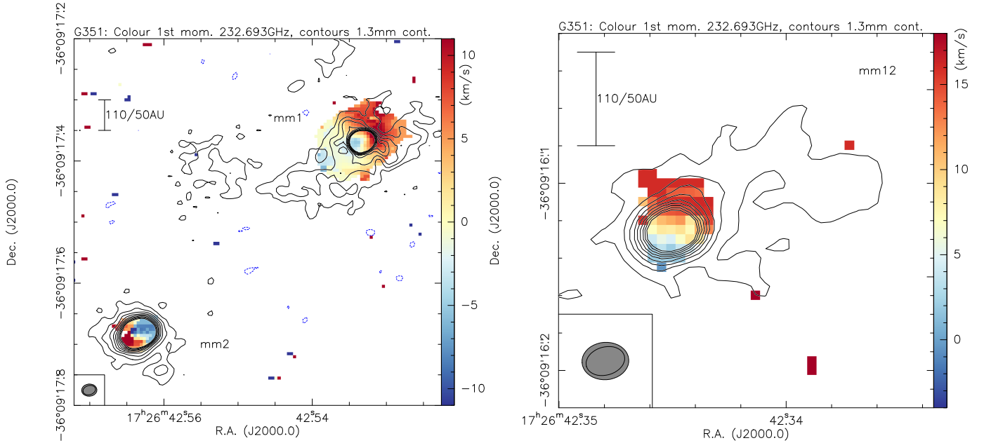
Fig. 8. Color-scale first moment maps (intensity-weighted peak velocities) from the line at 232.693 GHz. Left panel: focus on mm1 and mm2. Right panel: mm12. The contours are the 1.3 mm continuum data in 4\sigma level of 0.2 \text{ mJy beam}^{-1} up to a 3 \text{ mJy beam}^{-1} level (to avoid too many contours in the center). A scale-bar and the resolution elements of the line (gray) and continuum are shown as well.
