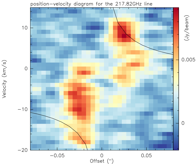
Fig. 5. Color-scale position-velocity diagram for mm1 for the line at 217.82 GHz along the axis of the strong velocity gradient visible in Fig. 3. The lines correspond to a Keplerian curve around a 10 M_{\odot} central object, not representing the data well.
