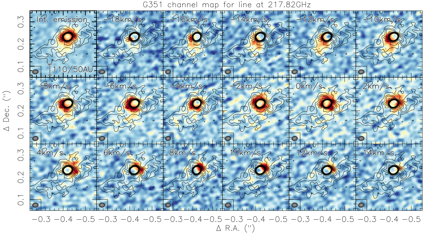
Fig. 4. Channel map of the 217.82 GHz line for mm1. Top-left panel: integrated emission between -18 and +14 \text{km s}^{-1} . The remaining panels show the channels with 2 \text{km s}^{-1} width at the velocities marked at the top-left of each panel. The contours are the 1.3 mm continuum data in 4\sigma level of 0.2 \text{mJy beam}^{-1} up to a 3 \text{mJy beam}^{-1} level (to avoid too many contours in the center). A scale-bar is shown in the top-left panel, and the resolution elements of the line (gray) and continuum are presented in each panel. The v_{\text{lsr}} is at approximately -3.6 \text{km s}^{-1} .
