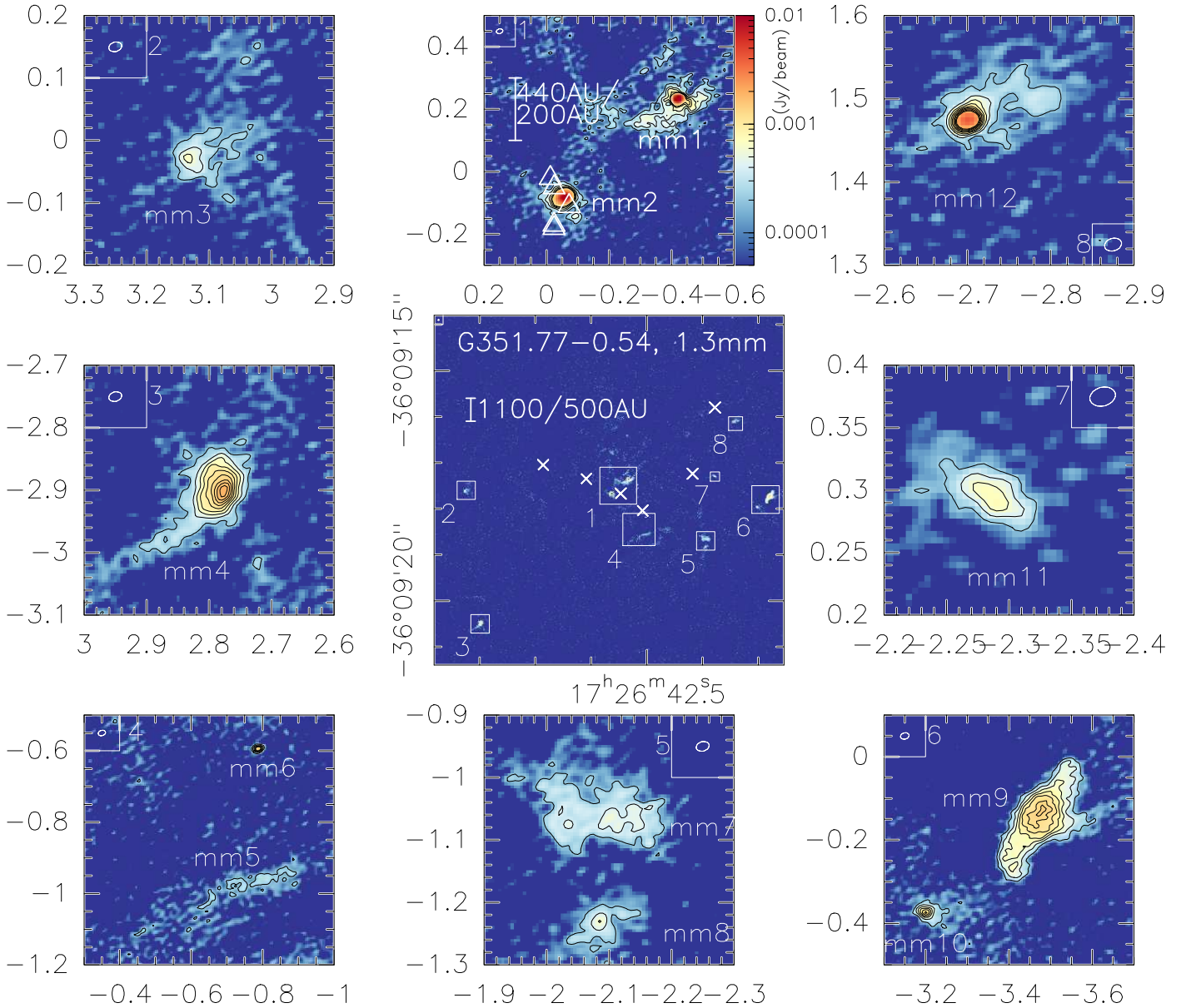
Fig. 2. ALMA 1.3 mm continuum data toward the high-mass star-forming region G351.77-0.54 at an angular resolution of 0.021'' \times 0.015'' . Central panel: overall structure (the white crosses mark the cm continuum source positions from Zapata et al. 2008), and the surrounding panels show selected zooms into the areas marked in the central panel. We note the different cutout sizes of the individual zoom windows. The contour levels always start at a 4\sigma level of 0.2 \text{ mJy beam}^{-1} and continue in 4\sigma steps. Scale bars assuming 1.0/2.2 \text{ kpc} distance are shown in the middle and middle top panels. Middle top panel: \text{CH}_3\text{OH} maser positions from Walsh et al. (1998) and an intensity scale. The synthesized beam is presented in each panel.
