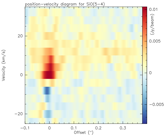
Fig. 7. Color-scale position–velocity diagram from SiO(5–4) along the outflow axis seen in Fig. 6.
