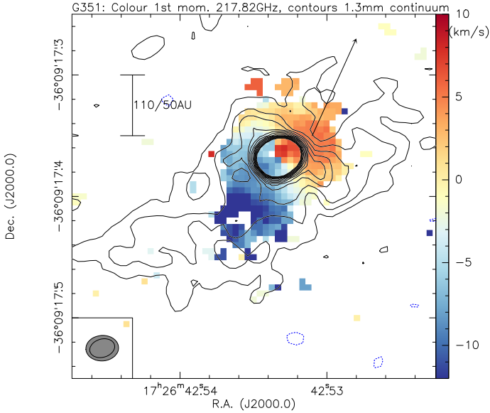
Fig. 3. Color-scale first moment map (intensity-weighted peak velocities) for mm1 from the line at 217.82 GHz. The contours are the 1.3 mm continuum data in 4\sigma levels of 0.2 \text{ mJy beam}^{-1} up to a 3 \text{ mJy beam}^{-1} level (to avoid too many contours in the center). A scale-bar and the resolution elements of the line (gray) and continuum are shown as well. The arrow outlines the approximate direction of the CO(6–5) red outflow lobe shown in Fig. 6.
