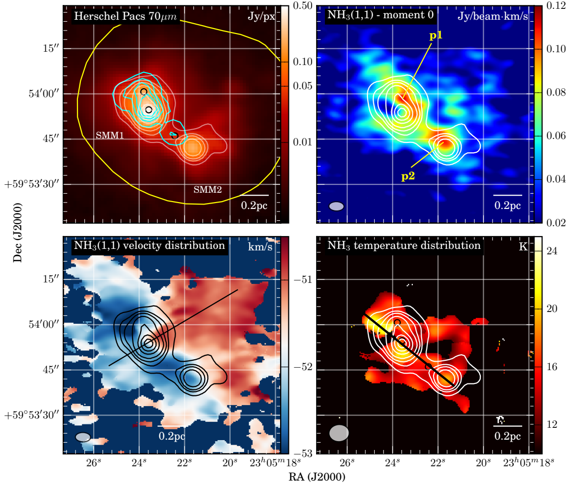
Fig. 6. ISOSS23053 – overview. Upper left panel: Herschel PACS 70\ \mu\text{m} emission, and cyan contours present Spitzer MIPS 24\ \mu\text{m} emission at levels of 75, 150, 225, and 300 MJy/sr. The yellow contour shows the 3-sigma limit of the SCUBA 850\ \mu\text{m} emission and therefore the area where we measured the clump mass. Following panels: VLA and Effelsberg 100 m Telescope data combined. Upper right panel: integrated emission of the main \text{NH}_3(1,1) line in \text{Jy beam}^{-1} \text{km s}^{-1} from -53.3 to -50.1\ \text{km s}^{-1} . Lower left panel: peak velocity distribution in \text{km s}^{-1} , and the black line indicates the direction of the position-velocity cut shown in Fig. 7. Lower right panel: kinetic temperature in K. We extracted the temperature distribution along the black line shown in the lower right panel and plotted the values as a function of distance in Fig. 10. The black circles indicate Spitzer MIPS 24\ \mu\text{m} emission sources. In each panel white/black contours present Herschel PACS 70\ \mu\text{m} emission at levels of 20, 40, 60, 100, 200, 300, and 400 mJy/pixel. The \text{NH}_3(1,1) emission peaks are marked in the upper right panel, and the corresponding spectra are given in Fig. A.6. The synthesized beam and scale are shown in each panel.
