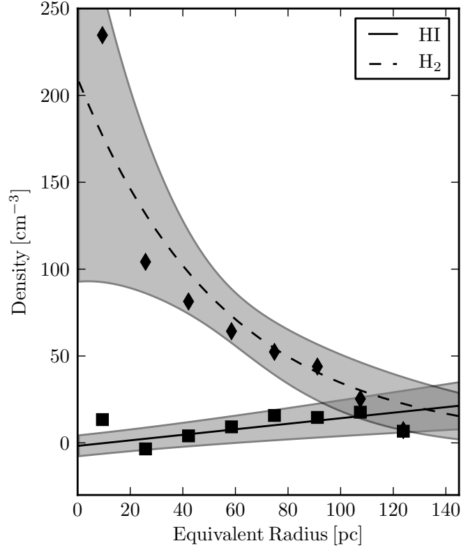
Fig. 14. Density of HI and \text{H}_2 as a function of the distance toward the center of W43 (equivalent radius). The diamonds and the dashed line represent the molecular hydrogen, whereas squares and the solid line represent the atomic hydrogen. The corresponding 3\sigma uncertainties from the fit introduced in Eq. (14) are shown as gray shaded areas.
