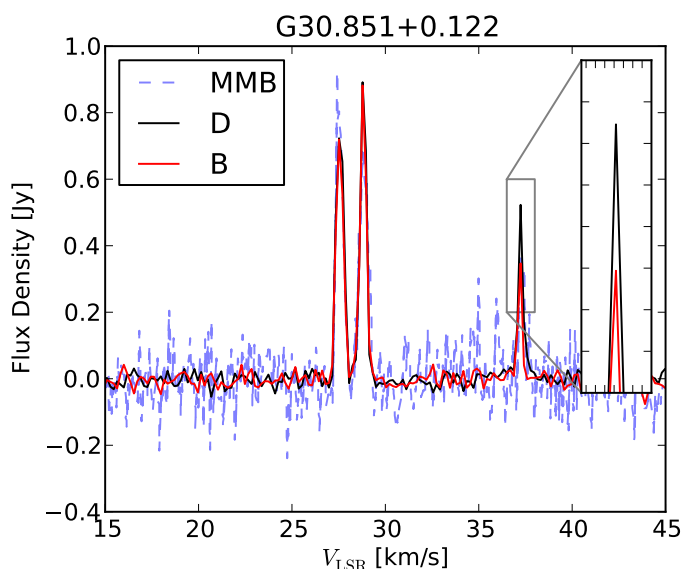
Fig. 10: Methanol maser spectra of source G30.851+0.122. Shown in solid lines are the GLOSTAR spectra in black and red for D-configuration and B-configuration, respectively. The dashed blue line is the MMB spectrum of the corresponding source. The zoom-in depicts the velocity component which shows a difference in intensity between the two configurations (it is spatially unresolved in both D- and B-configuration).
