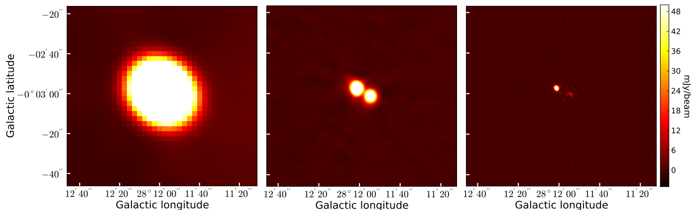
Fig. 8: From left to right images from D, D+B, and B-configuration images of G28.2-0.04.
