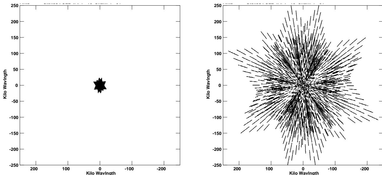
Fig. 2: The uv-coverage of a single source at high declination from the D-configuration (left) and B-configuration (right) observations. While both configurations probe very different ranges, there is significant overlap in the center that allows the combination into a single image. Note that part of this overlap is due to the large bandwidth covered by the observations.
