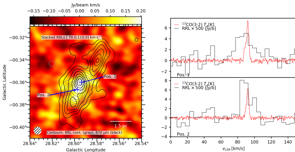
Fig. 13: Overview of the RRL emission of the HII region G28.59-0.364. The left panel shows integrated, stacked RRL emission at 25'' resolution. The GLOSTAR broadband 5.8 GHz continuum is shown in gray contours from -0.005 \text{ Jy beam}^{-1} in steps of 0.01 \text{ Jy beam}^{-1} . ATLASGAL 870 \mu m emission (Schuller et al. 2009) is shown in black contours starting from 0.2 \text{ Jy beam}^{-1} in steps of 0.2 \text{ Jy beam}^{-1} . ^{13}\text{CO} (3-2) emission from the CHIMPS survey (Rigby et al. 2016) is shown as red spectra on the right. All data have been smoothed to the angular resolution of the RRL data of 25''. The positions of extracted spectra in the side-panels are indicated with blue crosses.
