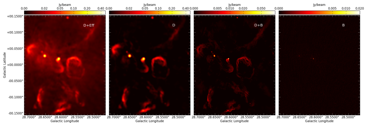
Fig. 6: Comparison of a smaller region between the D-configuration and Effelsberg combination (left), the D-configuration only image (middle left), the combination of D- and B-configurations (middle right), and the B-configuration image (right).
