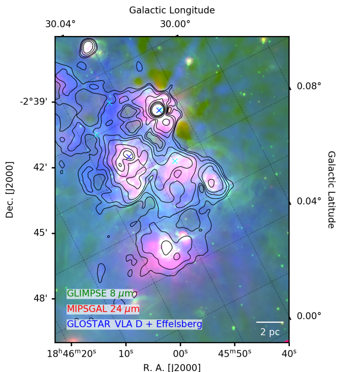
Fig. 14: Multi-color image of GLIMPSE 8 \mu\text{m} (green, Churchwell et al. 2009), MIPS GAL 24 \mu\text{m} (red, Carey et al. 2009) and GLOSTAR VLA D+Effelsberg 5.8 GHz emission (blue) of the G29.93-0.03 (W43-South) star formation complex. We use square-root scaling and truncate the individual datasets at 500 and 1000 MJy/sr for the 8 and 24 \mu\text{m} data, respectively, and at 20 mJy beam -1 for the cm-emission. Saturated pixels in the MIPS-GAL maps were replaced with the truncation value, accordingly. The data are shown in their native resolution. For reference, we overplot the markers from Fig. 15. The GLOSTAR 5.8 GHz data are repeated as contours for clarity, in steps of 15, 20, 30, 45, 100, 200, 300 and 500 mJy beam -1 .
