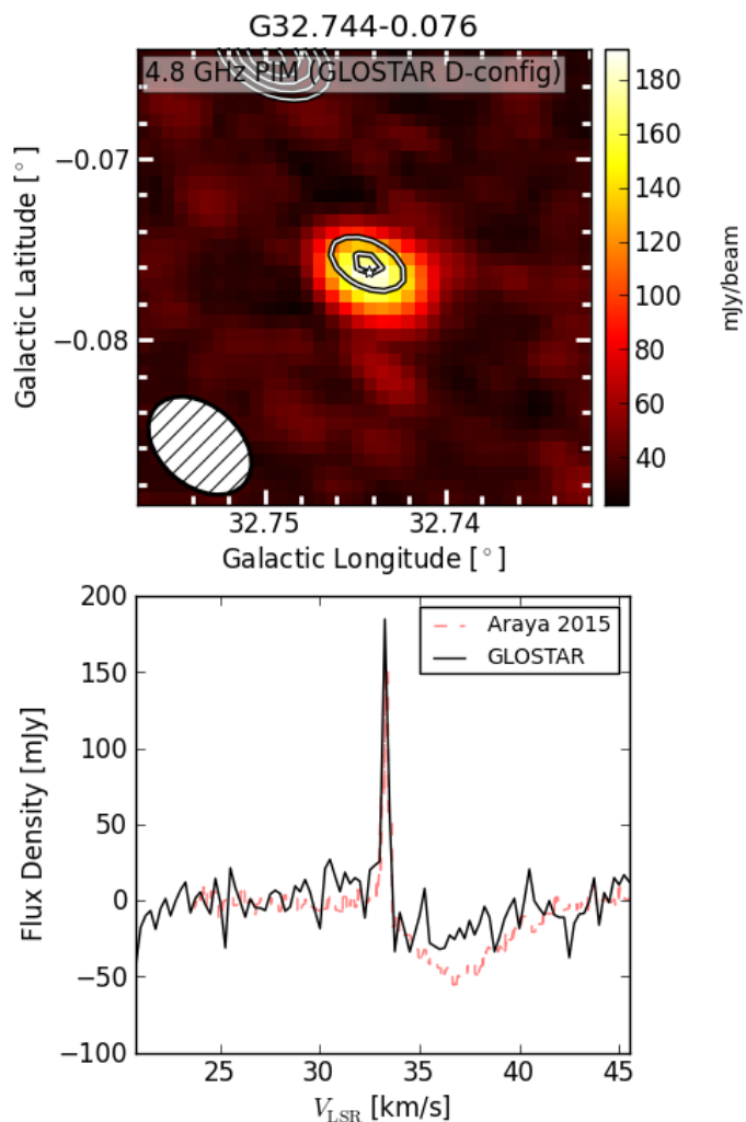
Fig. 11: Top : Peak intensity map of known 4.8 GHz formaldehyde maser G32.744-0.076 (Araya et al. 2015) using GLOSTAR VLA D-configuration data and the continuum emission as white contours. Bottom : Spectra extracted from GLOSTAR is shown as a solid black line and as a dashed red line from the Araya et al. (2015) paper. Despite our lower sensitivity, we can also faintly see the subsequent superimposed absorption feature.
