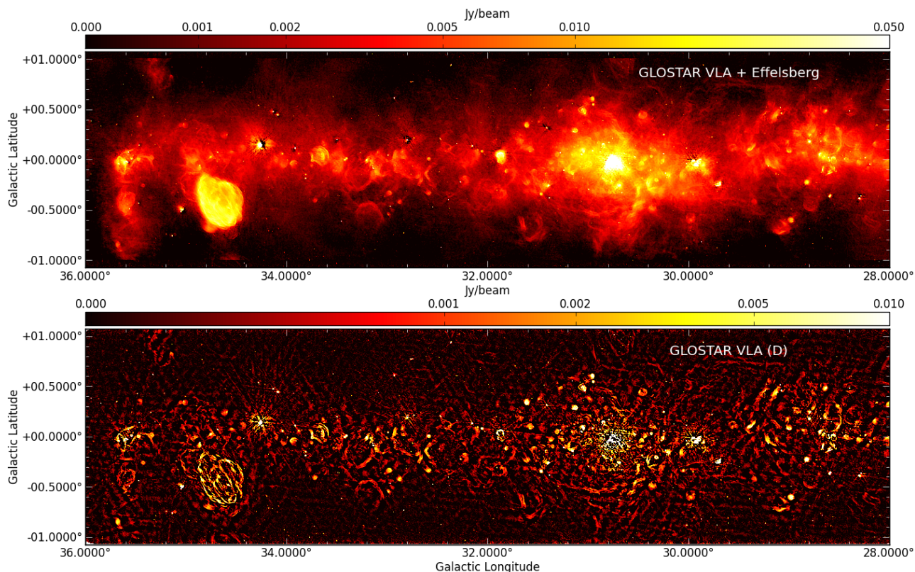
Fig. 4: Top: Continuum radio image of the pilot region in the range 28^\circ < l < 36^\circ from the combination of the VLA D-configuration and the Effelsberg single dish images. Bottom: D-configuration VLA image of the full continuum of the same longitude range which was already presented in Medina et al. (2019).
