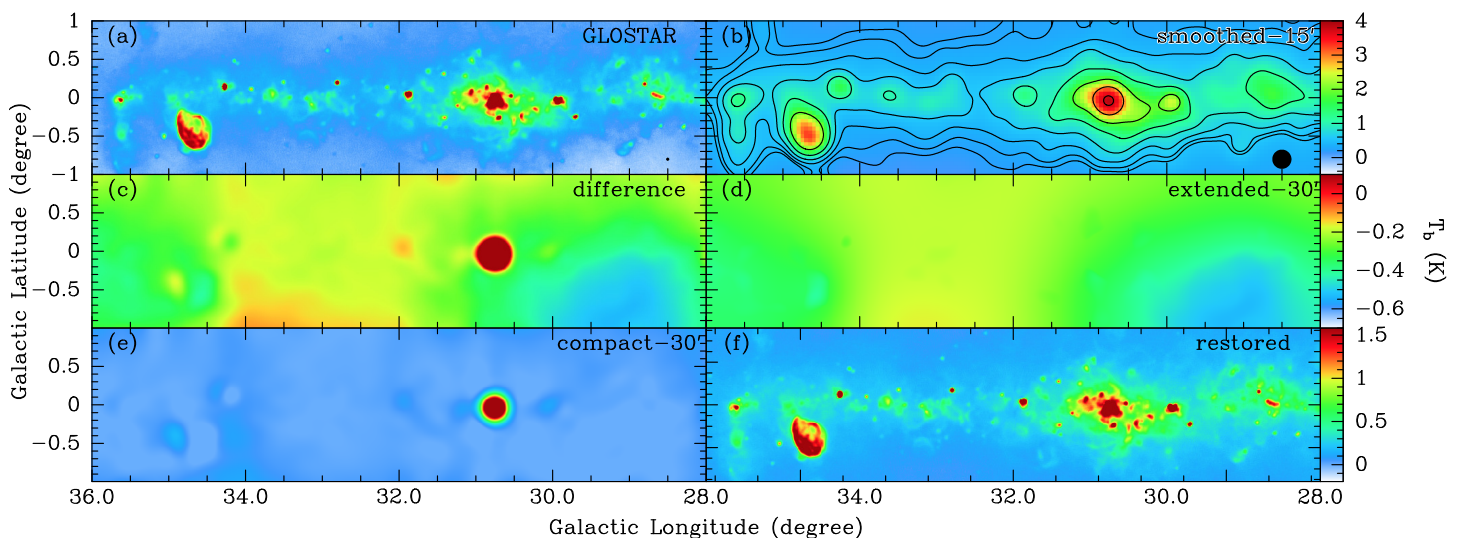
Fig. 3: (a) Effelsberg 4.8 GHz continuum image. (b) Urumqi 6 cm continuum emission overlaid with the Effelsberg 4.8 GHz continuum contours. Both datasets have been convolved to an angular resolution of 15' . The contours start at 50 mK, and each contour is twice the previous one. (c) Difference map derived by subtracting the Urumqi 6 cm continuum emission from the Effelsberg 4.8 GHz continuum map in Fig. 3b. (d) Extended emission component of Fig. 3c derived by the background filter method. (e) Compact emission component derived by the background filter method (f) Restored Effelsberg 4.8 GHz continuum image.
