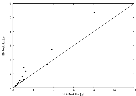
Fig. 5: Comparison of peak fluxes of several sources for the Effelsberg and VLA images. The solid line denotes a 1:1 ratio.
