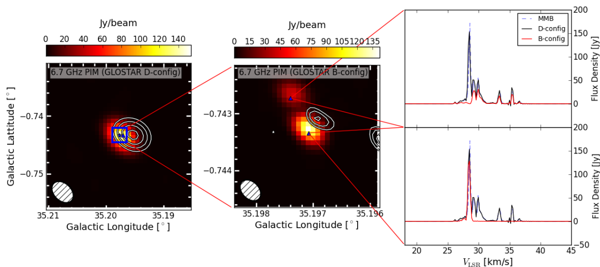
Fig. 9: Presented are peak intensity maps (PIM) over the velocity range of the methanol maser source G35.197-0.743 and spectra obtained from VLA data. On the left is the VLA D-configuration data, which has an average beamsize of \sim 18 arcsec. When observed in the B-configuration (with beamsize \sim 1.5 arcsec, middle panel), one can see that the higher resolution allows us to resolve the maser into two sources. Viewing the spectra on the right, we see that the first peak at 28.51 \text{ km s}^{-1} belongs only to the southern source while the rest belong to the northern source. The white contours mark the GLOSTAR radio continuum emission.
