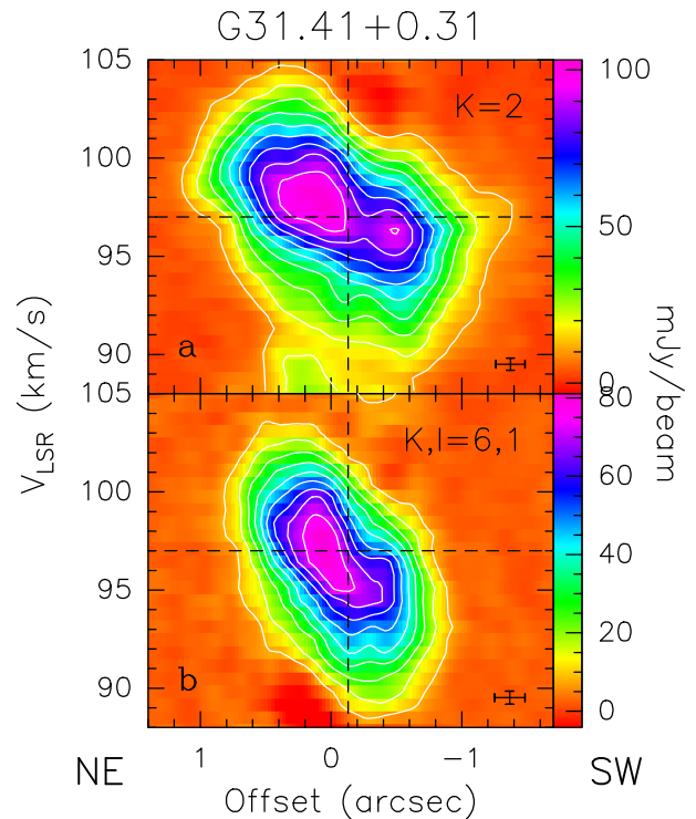
Fig. 19. a. PV plot of the ^{13}\text{CH}_3\text{CN}(13-12) K=2 line emission (excitation energy of 96 K) in G31.41 along a direction with \text{PA}=68^\circ passing through the HMC (dotted line in Fig. 9). The vertical and horizontal dashed lines indicate, respectively, the position of the continuum peak and the systemic velocity. The cross in the bottom right denotes the angular and spectral resolutions. b. Same as top panel, for the \text{CH}_3\text{CN}(12-11) v_8=1 K, l=6, 1 line (excitation energy of 778 K).
