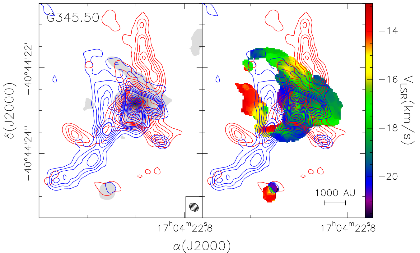
Fig. 15. Same as Fig. 13, for G345.50. The image in the right panel is the first moment of the 13 CH 3 CN(13–12) K=2 line. The SiO emission has been integrated over the velocity intervals -23.8 to -18.4 km s -1 and -15.7 to -10.3 km s -1 for the blue and red wings, respectively. Contour levels range from 4.2 to 29.4 in steps of 4.2 mJy/beam and from 30 to 130.8 in steps of 12.6 mJy/beam.
