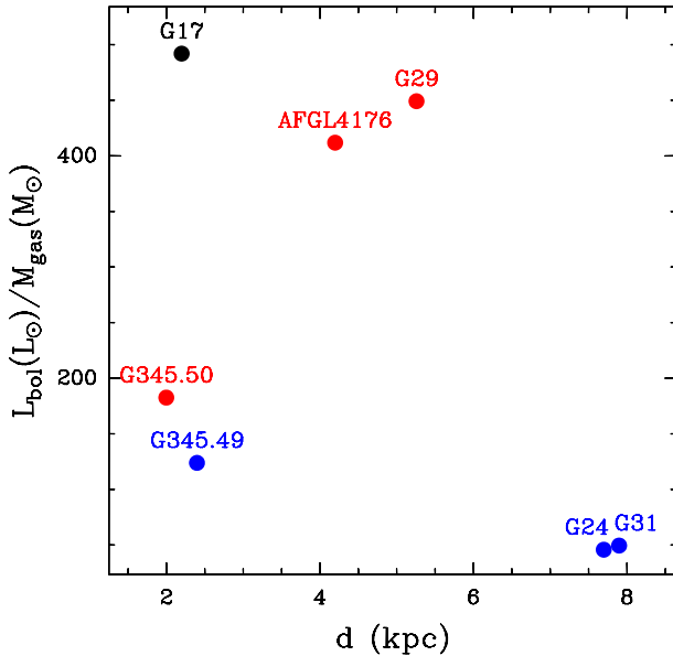
Fig. 29. Luminosity-to-mass ratio versus source distance for the 6 targets of our sample plus the disk around the 25 M_{\odot} star in AFGL 4176 detected by Johnston et al. (2015). Black, red, and blue points indicate, respectively, sources without evidence for disks, with disk candidates, and with questionable disk candidates (see Table 4).
