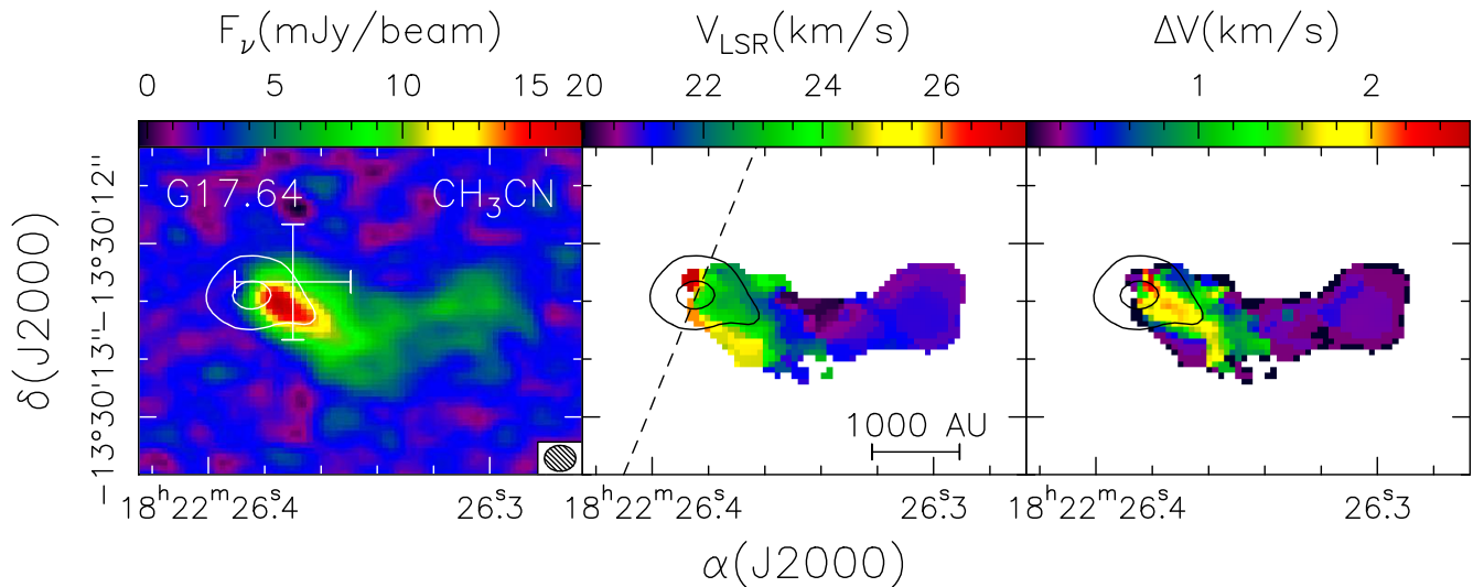
Fig. 6. Left. Map of G17.64 obtained by averaging the emission over the CH 3 CN(12–11) K=2 line. The contours correspond to the 5\sigma (outer contour) and 50% level (inner contour) of the continuum emission. The cross marks the position, with errors, of the centimeter continuum source detected by Menten & van der Tak (2004). The synthesised beam is shown in the bottom right. Middle. Same as left panel, for the 1st-moment map. The dashed line indicates the direction of the axis of the 12 CO outflow detected by Kastner et al. (1994). Right. Same as left panel, for the 2nd-moment map.
