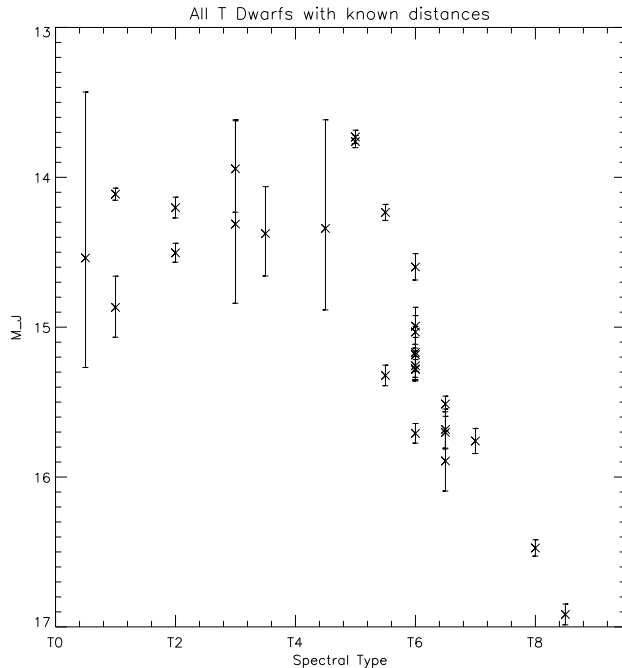
Figure 5. Absolute J magnitudes derived from all known T dwarf distances. 2MASS J magnitudes and spectral types taken from Burgasser (ref).
