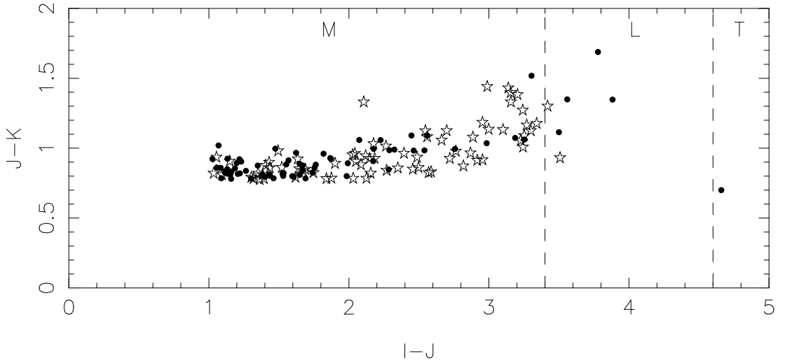
Figure 4.3: A two colour diagram showing objects found in the SIPS-I survey. The black dots are previously known objects and the stars are new discoveries.
