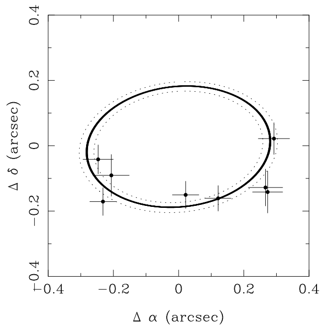
Figure 5.2: The parallax ellipse for the fitted value (solid line) found for SCR1845–6357 along with those for one sigma errors (dotted lines) plotted against the data.
