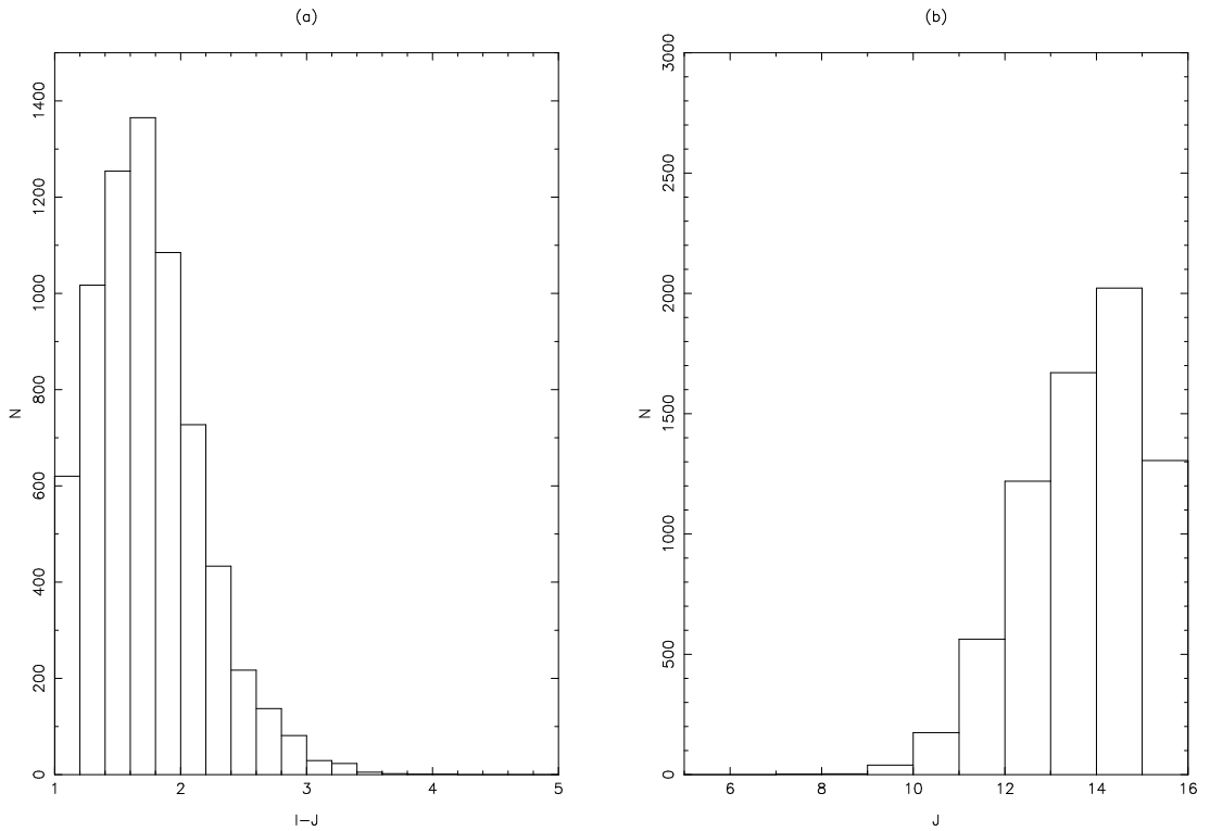
Figure 4.5: Histograms showing the magnitude ( J ) and colour ( I - J ) of the objects found in the SIPS-II survey (those with \mu < 0.5 ). The binning here is in smaller bins than in Figure 4.4 to allow more detailed comparison with the results of the simulations outlined in Chapter 6.
