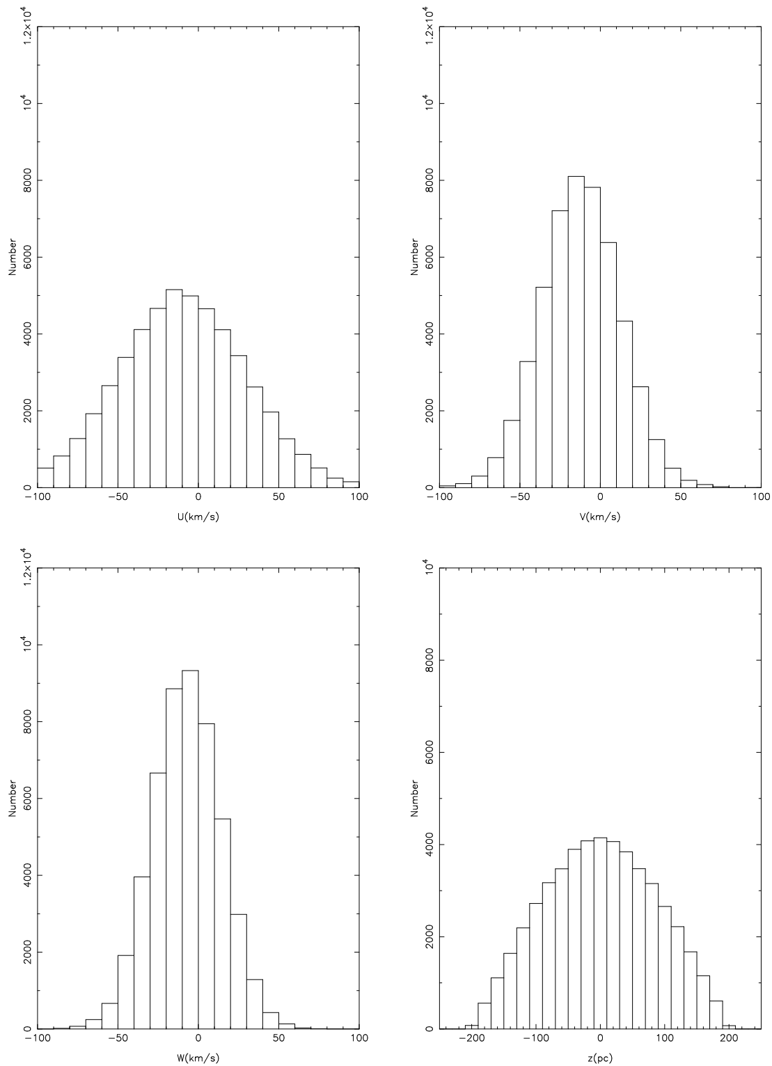
Figure 6.1: The simulated space velocities and position perpendicular to the Galactic Disk for 50,000 objects with ages ranging from 5-10 Gyr.
