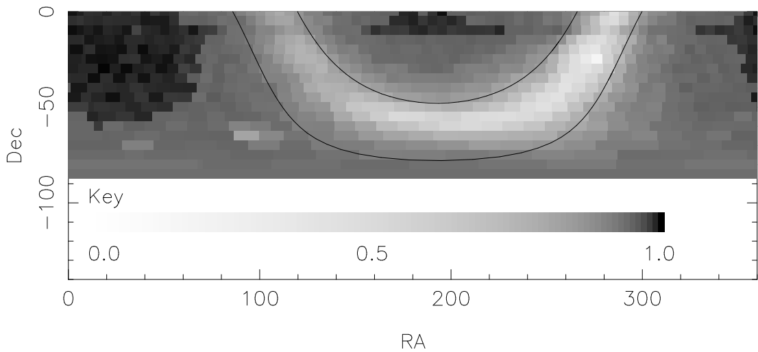
Figure 4.9: The areal completeness of the survey. The scale shows the probability that an area is free from both crowding and bright stars. The solid lines marked represent the galactic latitude cut of |b| > 15^\circ .
