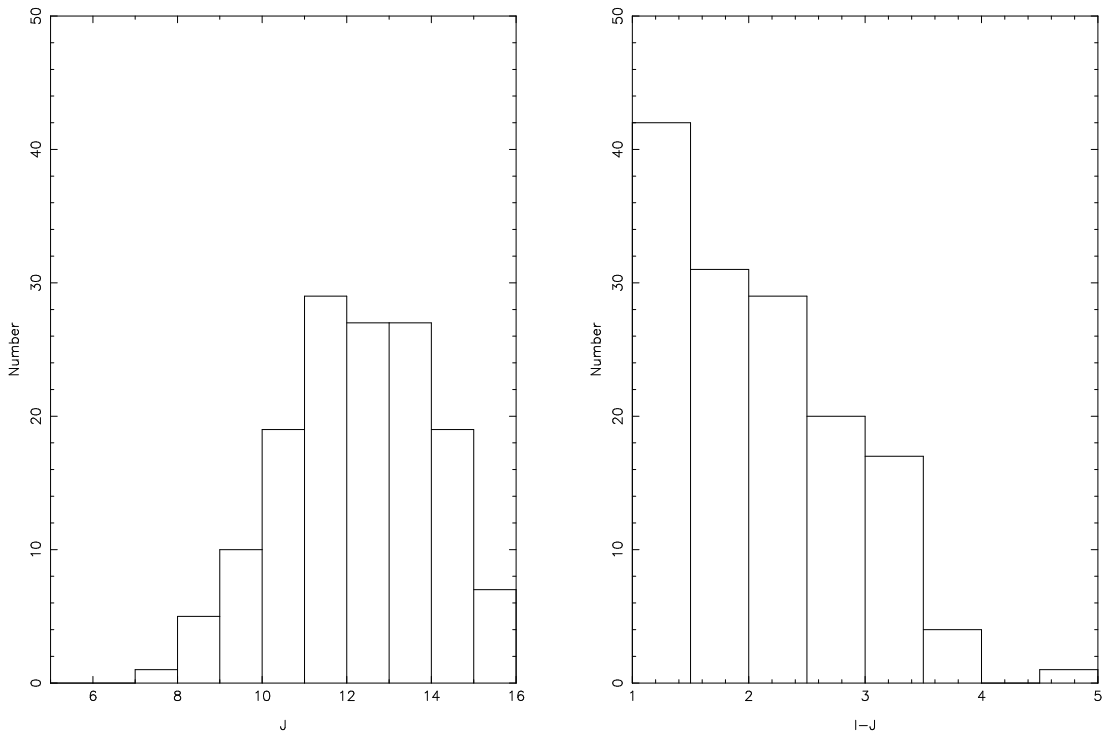
Figure 4.4: Histograms showing the magnitude ( J ) and colour ( I - J ) of objects found in the SIPS-I survey (those with \mu > 0.5''/\text{yr} ).
