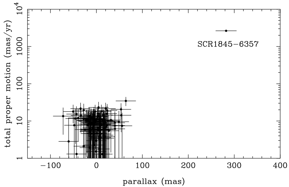
Figure 5.3: The parallaxes and proper motions for the reference stars and SCR1845-6357. It is clear that SCR1845-6357 is well separated from the mass of reference stars.
