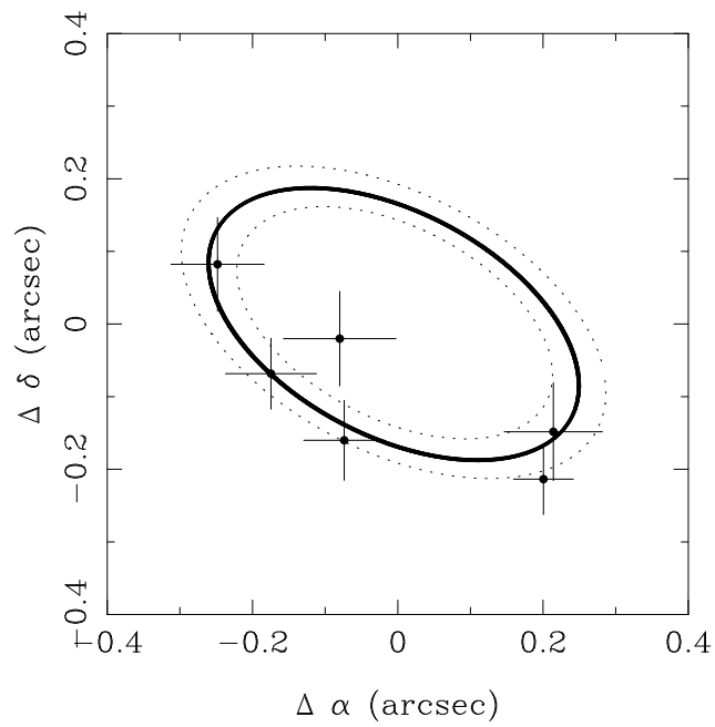
Figure 5.5: The parallax ellipse for the fitted value (solid line) for SIPS1259–4336 along with those for one sigma errors (dotted lines) plotted against the data.
