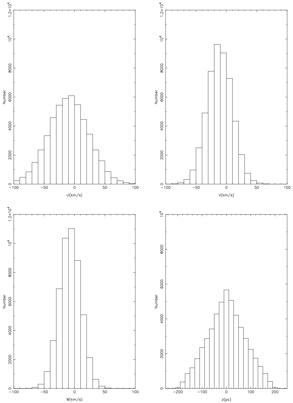
Figure 6.2: The simulated space velocities and position perpendicular to the Galactic Disk for 50,000 objects with ages ranging from 0-5 Gyr.
