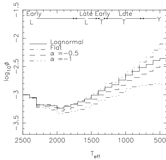
Figure 6.6: The alteration to the effective temperature distribution caused by different underlying IMFs. In this case a constant birthrate is used and the simulations are all normalised to the same point in the hottest bin. Note that the main effect is the height of the second peak. The temperature regions corresponding to each spectral type are taken from Vrba et al. (2004).
