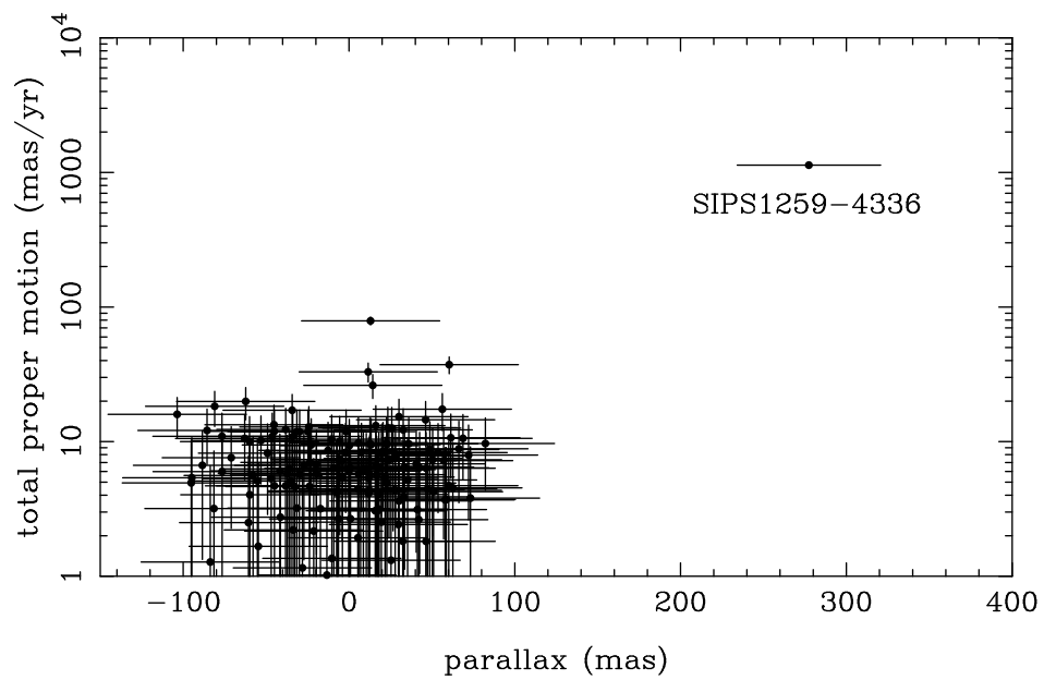
Figure 5.6: The parallaxes and proper motions for the reference stars and SIPS1259-4336. It is clear that SIPS1259-4336 is well separated from the mass of reference stars.
