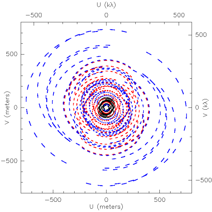
Fig. A.3. Simulated uv-coverage.
