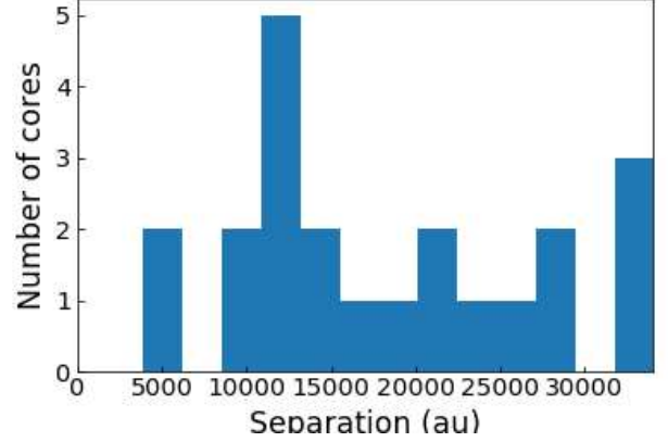
Fig. 5. Nearest-neighbor separation histogram from minimum spanning tree analysis for both regions combined. The spatial resolution limits are \sim 2700 and \sim 3500 au for ISOSS22478 and ISOSS23053, respectively.
