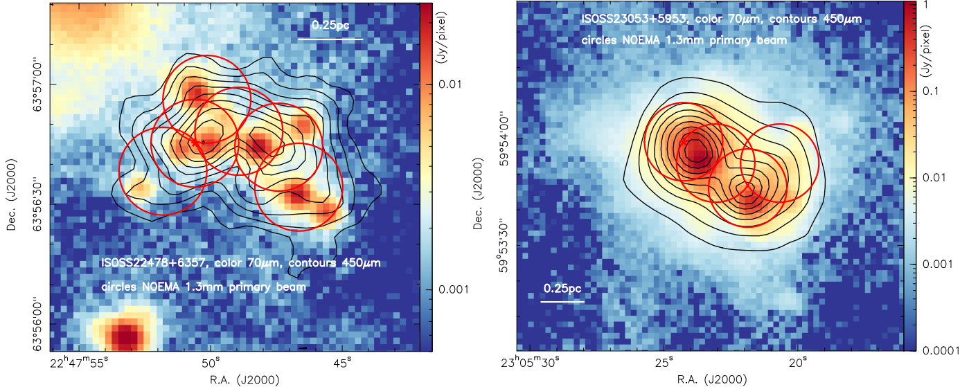
Fig. 1. Overview of the ISOSS22478+6357 (left) and ISOSS23053 (right) regions. The color scales and contours show the 70 and 450 \mu\text{m} emission from Herschel and SCUBA, respectively (Ragan et al., 2012; Di Francesco et al., 2008). The contour levels are from 18 to 98% of the peak emission of 1.88 Jy beam ^{-1} and 14.88 Jy beam ^{-1} for the two regions, respectively. Linear scale bars are shown and the red circles outline the NOEMA mosaics with a primary beam FWHM of 22".
