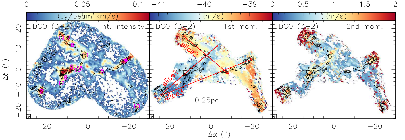
Fig. 6. NOEMA+30 m \text{DCO}^+(3-2) data towards ISOSS22478. The three panels show, in color scale the integrated intensity, the 1st and 2nd moment maps (intensity-weighted peak velocities and velocity dispersions), respectively. These maps were produced by clipping all data below an approximate 3\sigma threshold of 18 \text{ mJy beam}^{-1} . The contours show the 1.3 mm continuum emission in 3\sigma steps ( 1\sigma \sim 0.057 \text{ mJy beam}^{-1} ) from 3 to 15\sigma . The beam is shown in the bottom-left of all panels, and a linear scale bar is shown in the middle panels. The red arrows in the middle panel show the three position velocity slices presented in Fig. 8. To reduce noise signatures at the edges of the mosaic, for the 1st and 2nd moment maps, we blanked the mosaic edges. The cores are labeled in the left panel.
