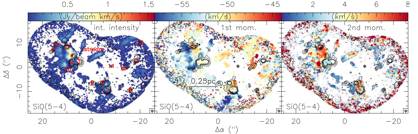
Fig. 13. NOEMA+30 m \text{SiO}(5-4) data towards ISOSS23053. The three panels show in color scale the integrated intensity, 1st and 2nd moment maps (intensity-weighted peak velocities and velocity dispersions), respectively. These maps were produced by clipping all data below an approximate 4\sigma threshold of 20 \text{ mJy beam}^{-1} . The contours show the 1.3 mm continuum emission in 3\sigma steps ( 1\sigma \sim 0.16 \text{ mJy beam}^{-1} ). The beam is shown in the bottom-right of all panels, and a linear scale bar is shown in the middle panel. The cores are labeled in the left panel. The arrow in the middle panel marks the position-velocity cut presented in Fig. 14.
