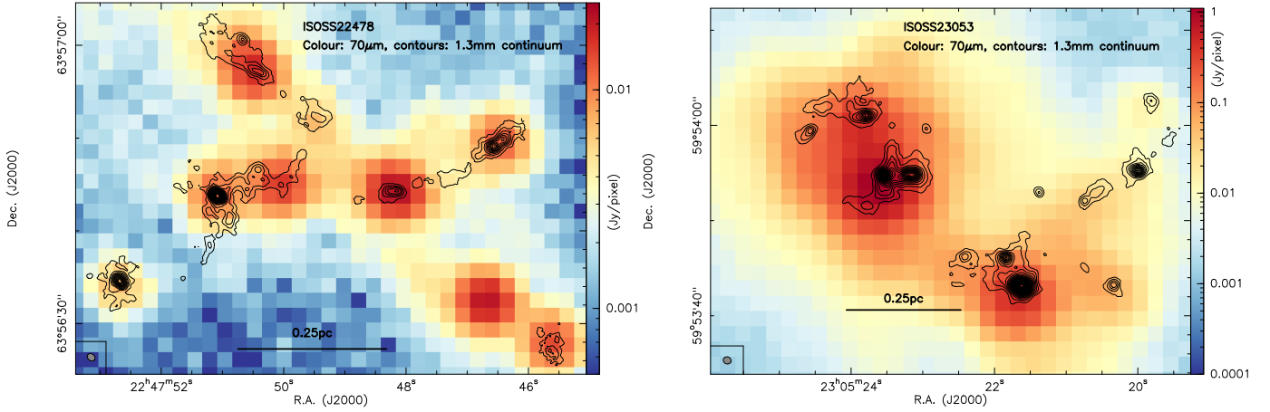
Fig. 2. NOEMA 1.3 mm continuum data for ISOSS22478 (left) and ISOSS23053 (right). The color scales show the 70\mu\text{m} Herschel data and the contours present the 1.3 mm NOEMA continuum data. The contour levels are in steps of 3\sigma with the 1\sigma level of 57\mu\text{Jy beam}^{-1} for ISOSS22478 and 160\mu\text{Jy beam}^{-1} for ISOSS23053. Linear scale bars and the 1.3 mm beam size are shown.
