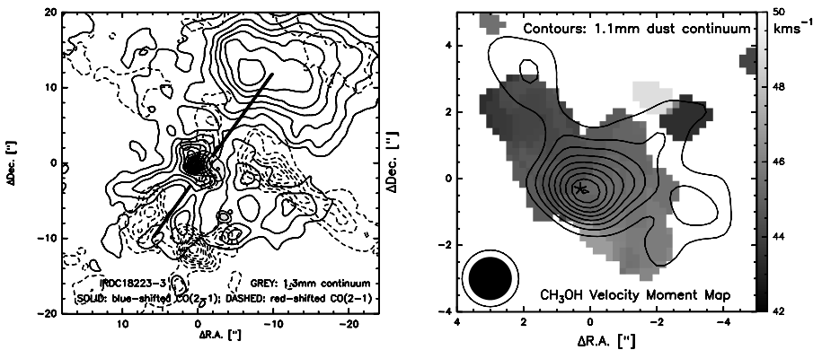
Figure 3: SMA observations toward IRDC 18223-3 (Fallscheer et al. in prep.). The left panel shows the blue- and red-shifted CO(2–1) emission as solid and dashed contours overlaid on the grey-scale 1.3 mm dust continuum emission. The central core is the same source as in Fig. 2. The right panel presents in grey-scale a 1st moment map (intensity weighted velocity distribution) of CH 3 OH overlaid with the 1.1 mm continuum emission. The empty and full circle are the synthesized beams of the line and continuum emission, respectively.
