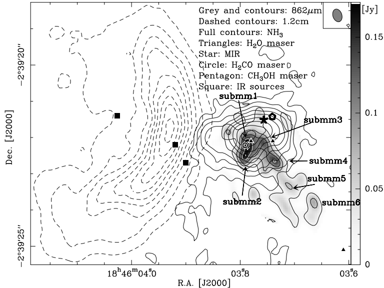
Figure 7: Compilation of data toward the UCHII/hot core region G29.96 from Beuther et al. 2007c. The dashed contours toward the cometary UCHII regions whereas the full contours show the older NH 3 observation from the hot core (Cesaroni et al. 1994). The grey-scale with contours then present the new high-resolution ( 0.36'' \times 0.25'' ) submm continuum data from the SMA.
