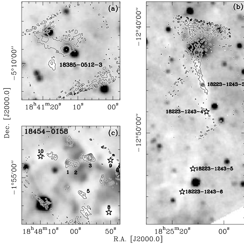
Figure 1: Sample IRDCs from Sridharan et al. (2005): MSX A-band ( 8\ \mu\text{m} ) images (black is bright) with 1.2 mm emission contours: The first two numbers refer to the corresponding IRAS source and the third number labels the mm sub-sources. The five-pointed stars mark cores lacking good 1.2 mm measurements.
