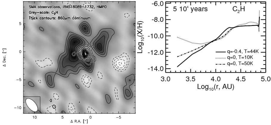
Figure 10: The left panel presents in grey-scale the C_2H emission and in thick solid contours the corresponding submm continuum from the SMA toward the HMPO IRAS 18089-1732 (Beuther et al., subm. ). The right panel shows a chemical model explaining the decreased emission toward the core center after approximately 5 \times 10^4 yrs. The parameter q denotes the temperature power-law index, and the T values refer to the temperature at the core edge or to isothermal values ( q = 0 ).
