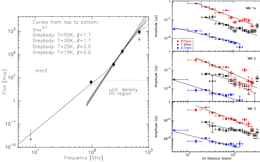
Figure 8: The left panel presents the SED toward the coldest sub-source in IRAS 05358+3543 (Beuther et al. 2007b). The parameters of the fits are marked in the figure. The right panel shows intensities averaged in uv-annuli and plotted versus the baseline-length for different sub-sources and wavelengths. Most can be well fitted by power-law distributions.
