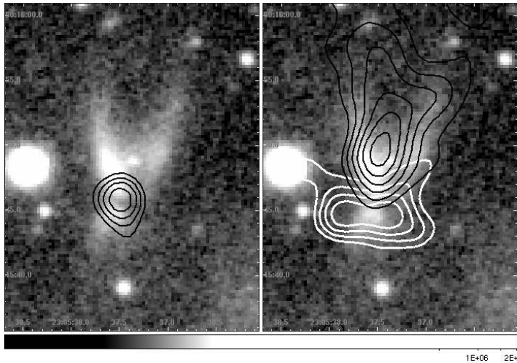
Figure 5: The grey-scale in both panels shows the K-band near-infrared nebulosity observed for this massive evolved disk candidate (Quanz et al. in prep.). The contours are the corresponding SMA mm observations where the left panel shows the 1.3 mm continuum emission, and the right panel in black and white contours the blue-shifted ^{12}\text{CO}(2-1) and the integrated \text{C}^{18}\text{O}(2-1) emission, respectively.
