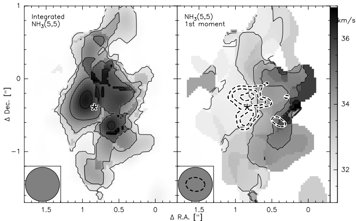
Figure 4: The left panel shows the VLA \text{NH}_3(5,5) emission integrated from 31 to 37 \text{ km s}^{-1} (Beuther & Walsh 2008). The right panel presents the corresponding 1st moment map contoured from 31.5 to 36.5 \text{ km s}^{-1} (step 1 \text{ km s}^{-1} ). The white-black dashed contours show the 1.2 cm continuum emission. The asterisks mark the position of the submm continuum peak (Beuther et al. 2005c), and the synthesized beams are shown at the bottom-left (grey \text{NH}_3 and dashed 1.2 cm emission).
