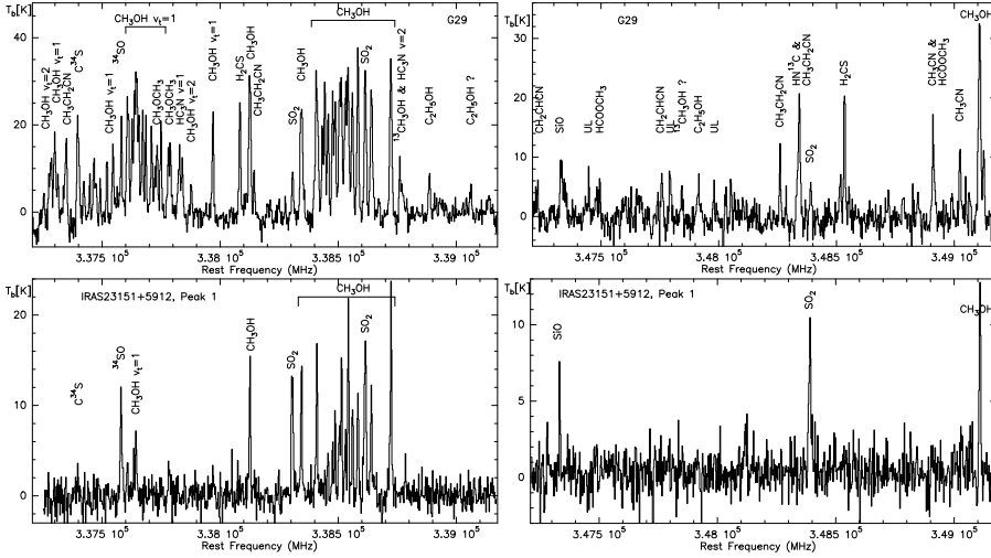
Figure 9: SMA spectra extracted toward two massive star-forming regions (G29.96 top row & IRAS 23151+5912 bottom row, Beuther et al., subm. ). The spectral resolution in all spectra is 2 km/s. The left and right column show the lower and upper sideband data, respectively.
