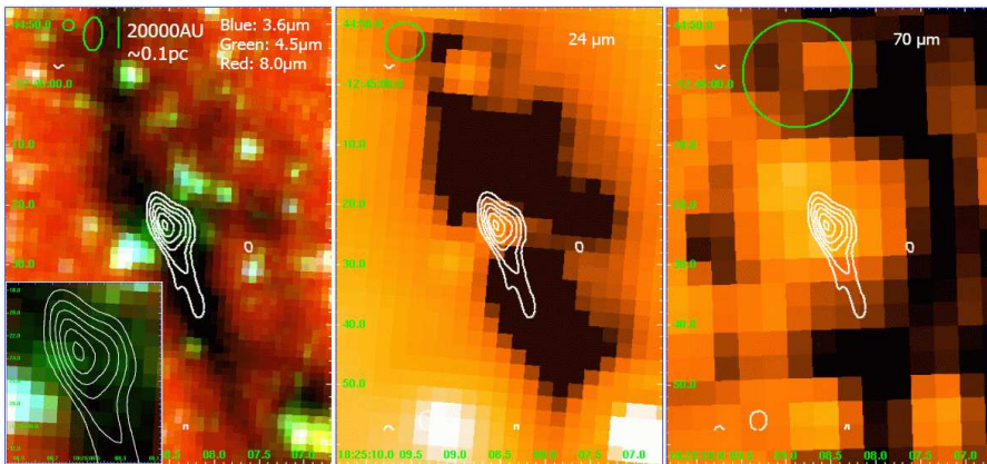
Figure 2: IRDC 18223-3 images at different wavelengths from Beuther & Steinacker (2007). The color scales show Spitzer images at various wavelength, and the contours show the 93 GHz (3.2mm) continuum emission observed with the PdBI (Beuther et al. 2005a). The left panel presents a three-color composite with blue 3.6 \mu\text{m} , green 4.5 \mu\text{m} and red 8.0 \mu\text{m} (adapted from Beuther et al. 2005a). The inlay zooms into the central core region. The middle and right panel show the Spitzer 24 and 70 \mu\text{m} images, respectively. The circles in each panel present the Spitzer beam sizes and the ellipse in the left panel presents the PdBI 3.2 mm continuum synthesized beam. A size-ruler is also shown in the left panel.
