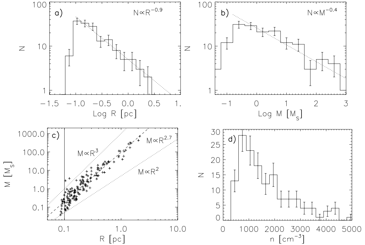
Fig. 2. Characteristics of the structures (clumps) defined by a thresholding at A_V^{\text{tail}} (see Sect. 3.1.1 in text). a) The size distribution. Error bars show the \sqrt{n} uncertainty. The dotted line shows the least-squares fit to the distribution, with the slope -0.9 \pm 0.2 . b) The same for the mass distribution. The linear fit results in the slope -0.4 \pm 0.2 . c) The mass-radius relation. Overplotted are slopes indicating M \propto R^3 and M \propto R^2 (dotted lines), the linear fit to the data points which has a slope 2.7 \pm 0.2 (dashed line), and the resolution limit R = 0.1 pc of the data (solid line). d) The distribution of mean volume densities.
