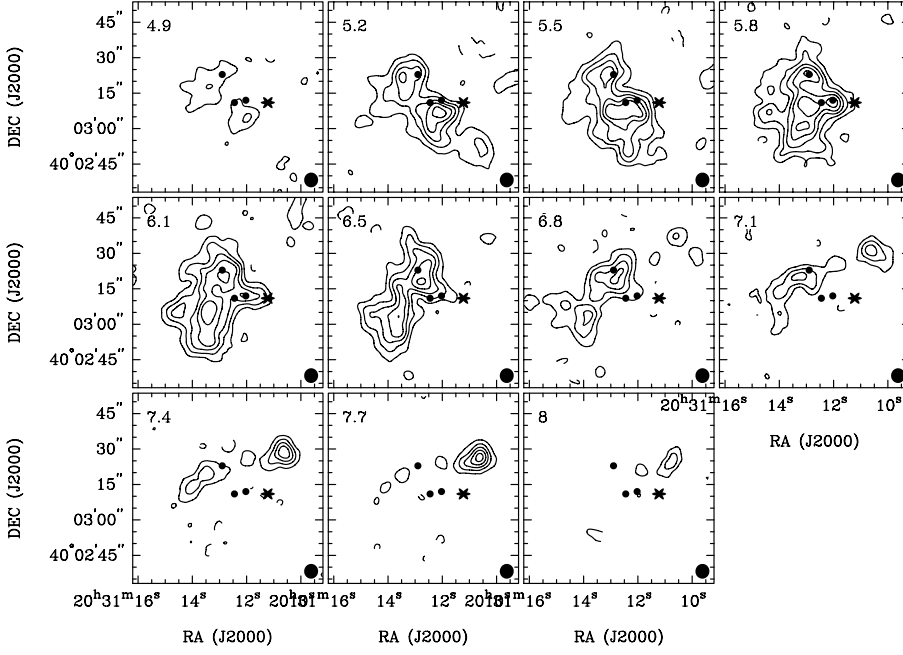
Fig. 7. N_2H^+ (1–0) channel maps for the F_1 = 0-1 hyperfine toward IRAS 20293+3952. Contour levels are -4, 4, 8, 12, 16, and 20 times the rms noise of the maps, 0.07 \text{ Jy beam}^{-1} . Filled circles are the compact millimeter sources detected by Beuther et al. (2004b), and the star marks the position of the UCH II region. The synthesized beam is shown in the bottom right corner.
