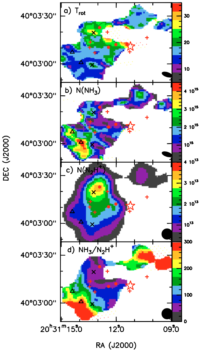
Fig. 10. a) Rotational temperature map from NH 3 (1, 1) and NH 3 (2, 2) obtained for the main cloud and the western cloud of the IRAS 20293+3952 region. Scale units are in K. b) NH 3 column density map. Scale units are in cm -2 . c) N 2 H + column density map convolved to an angular resolution of 7''. Scale units are in cm -2 . d) N(NH 3 )/N(N 2 H + ) ratio map after convolving the NH 3 column density map from panel b) to a final angular resolution of 7''. Symbols are the same as in Fig. 2. Beams are shown in the bottom right corner, and are 6''.9 × 3''.0, with PA = 71°.5 for panels a) and b) , and 7'' for panels c) and d) .
