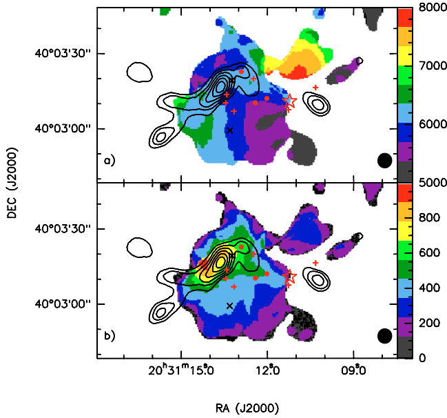
Fig. 8. a) Color scale: first-order moment map for the hyperfine F_1 = 0-1 line of N_2H^+ (1–0) toward IRAS 20293+3952. b) Color scale: second-order moment map for the hyperfine F_1 = 0-1 line of N_2H^+ (1–0). In both figures black contours are the same as Fig. 2a, showing the CH_3OH (2–1) emission, with contours starting at 13%, and increasing in steps of 15% of the peak intensity. Color scales are in \text{m s}^{-1} . The synthesized beam is shown in the bottom right corner, and symbols are the same as in Fig. 2. Note that the second-order moment gives the velocity dispersion, and must be multiplied by the factor 2\sqrt{2\ln 2} \approx 2.35 to obtain FWHM line widths.
