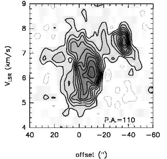
Fig. 9. N_2H^+ p-v plot for the F_1 = 0-1 hyperfine at PA = 110^\circ , that is, along the western cloud and the northern side of the main cloud. Central position is \alpha(J2000) = 20^{\text{h}}31^{\text{m}}13^{\text{s}}.63 ; \delta(J2000) = +40^\circ03'16''.7 (methanol peak), and positive position offsets are toward southeast. Contours start at 0.15 \text{ Jy beam}^{-1} , increasing in steps of 0.15 \text{ Jy beam}^{-1} .
