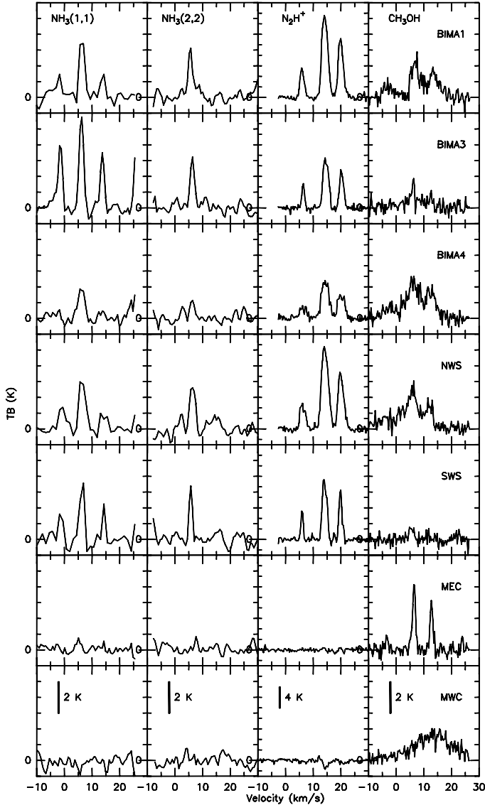
Fig. 3. Spectra toward seven positions of the IRAS 20293+3952 region for the four transitions studied in this paper, from left to right, \text{NH}_3(1, 1) , \text{NH}_3(2, 2) , \text{N}_2\text{H}^+(1-0) , and \text{CH}_3\text{OH}(2-1) . The seven positions are labeled on the right panel of each row, and are, from top to bottom, BIMA 1, BIMA 3, BIMA 4, NWS (Northern Warm Spot), SWS (Southern Warm Spot), MEC (methanol eastern clump), and MWC (methanol western clump). The vertical scale is indicated for each transition in the bottom row. For \text{CH}_3\text{OH} we show, in order of increasing velocity, the 2_0-1_0 E, 2_0-1_0 A + , and 2_{-1}-1_{-1} E lines (velocities are referred to the 2_0-1_0 A + line). For \text{N}_2\text{H}^+ , velocities are referred to the F_1 = 0-1 hyperfine.
