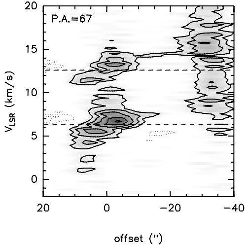
Fig. 6. \text{CH}_3\text{OH} p-v plot along outflow A, with PA = 67^\circ . Contours are -0.25, -0.15, 0.15, 0.25, 0.35, 0.45, and 0.52 \text{ Jy beam}^{-1} . The velocity resolution is 0.30 \text{ km s}^{-1} , and the channel maps have been convolved with a beam of 10'' \times 5'' , with a PA perpendicular to the direction of the cut, in order to recover the maximum emission in each position. The velocity range includes two lines: 2_0-1_0 \text{ A}^+ (at 6.3 \text{ km s}^{-1} , bottom dashed line) and 2_{-1}-1_{-1} \text{ E} (at 12.6 \text{ km s}^{-1} , top dashed line). The zero position corresponds to mm1, and positive values go to the northeast.
