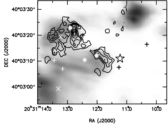
Fig. 11. Zero-order moment map of the \text{CN}(1-0) emission (contours) from Beuther et al. (2004b) in the IRAS 20293+3952 region, overlaid on the \text{NH}_3(1,1) emission shown in Fig. 2c (grey scale). \text{CN}(1-0) emission has been integrated from 4 to 12 \text{ km s}^{-1} , and contours start at 15% of the peak intensity, 273 \text{ Jy beam}^{-1} \text{ km s}^{-1} , increasing in steps of 15%. Symbols are the same as in Fig. 2. Beams are 6''.9 \times 3''.0 , with \text{PA} = 72^\circ for \text{NH}_3(1,1) , and 1''.46 \times 1''.21 , with \text{PA} = 32^\circ for \text{CN}(1-0) .
