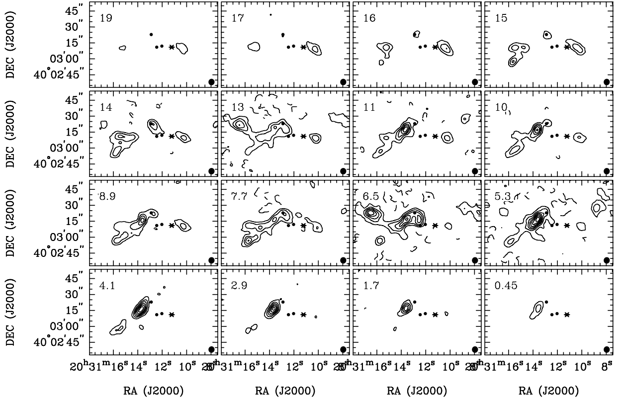
Fig. 4. \text{CH}_3\text{OH} channel maps toward IRAS 20293+3952 for the lines 2_0-1_0 A^+ (around 6.3 \text{ km s}^{-1} , the systemic velocity), and 2_{-1}-1_{-1} E (around 13 \text{ km s}^{-1} ), averaged every 4 channels. Contours are -16, -12, -8, -4, 4, 8, 12, 16, 20, 24, 28, and 32 times the rms of the map, 0.04 \text{ Jy beam}^{-1} . Filled circles are the compact millimeter sources detected by Beuther et al. (2004b), and the star marks the position of the UCH II region. The synthesized beam is shown in the bottom right corner of each panel.
