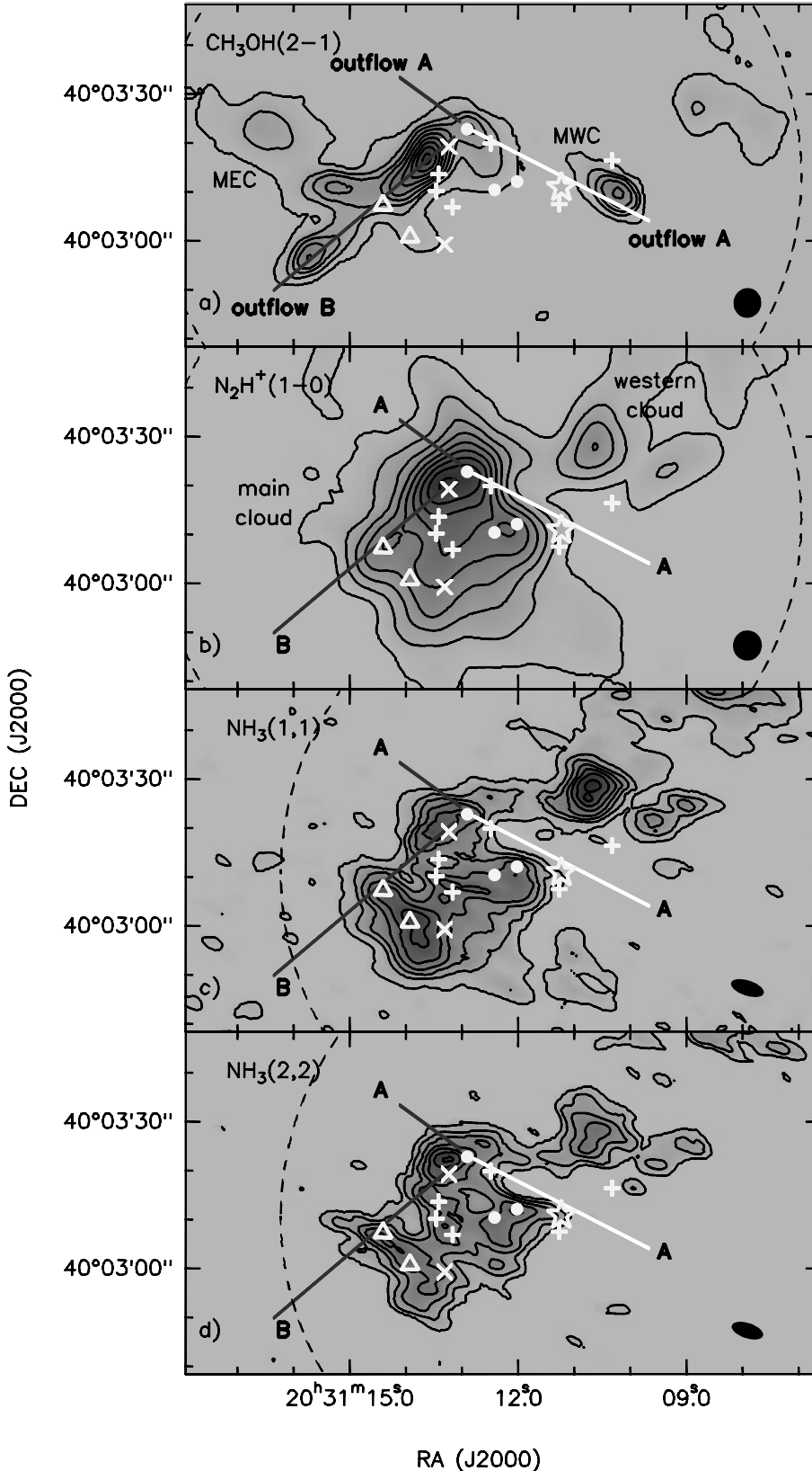
Fig. 2. a) \text{CH}_3\text{OH} zero-order moment for the 2_0-1_0 A^+ , and 2_{-1}-1_{-1} E lines toward IRAS 20293+3952. Contours start at 1%, increasing in steps of 12% of the peak intensity, 10.7 \text{ Jy beam}^{-1} \text{ km s}^{-1} . b) \text{N}_2\text{H}^+ zero-order moment integrated for all the hyperfine components of the (1–0) transition. Contours start at 2%, increasing in steps of 12% of the peak intensity, 21.9 \text{ Jy beam}^{-1} \text{ km s}^{-1} . c) \text{NH}_3 (1, 1) zero-order moment. Contours start at 5%, increasing in steps of 15% of the peak intensity, 0.240 \text{ Jy beam}^{-1} \text{ km s}^{-1} . d) \text{NH}_3 (2, 2) zero-order moment. Contours start at 7%, increasing in steps of 15% of the peak intensity, 0.0892 \text{ Jy beam}^{-1} \text{ km s}^{-1} . In all panels, the first level is about 3 times the rms noise of the map. Symbols are the same as in Fig. 1, with the star marking the peak of the centimeter emission, and the triangles marking the positions of BIMA 3 and BIMA 4 cores. MEC and MWC stand for methanol eastern clump and methanol western clump, respectively. The synthesized beams for each transition are shown in the bottom right corner, and are listed in Table 1. The straight lines mark the direction of outflows A and B (Beuther et al. 2004a), with the light grey line corresponding to the redshifted lobe. The dashed curve indicates the primary beam of BIMA (panels a) and b)) and VLA (panels c) and d)) observations.
