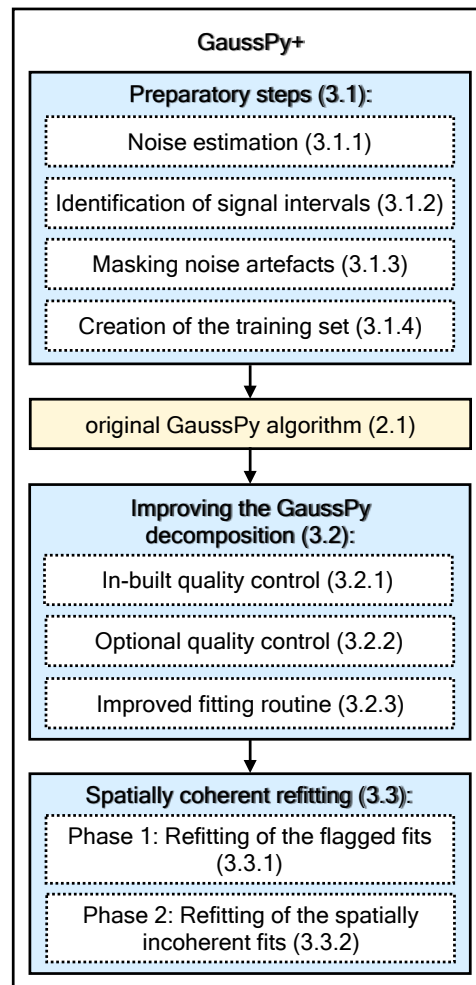
Fig. 1. Schematic outline describing new automated methods and procedures included in GAUSSPY+, along with corresponding sections in this paper.
