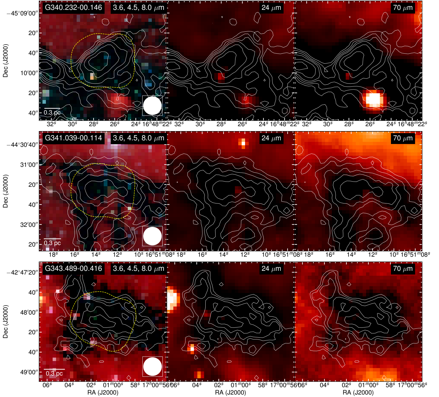
Figure 4. Same as in Figure 1, except for contour levels for the 870\ \mu\text{m} dust continuum emission, which are: 3, 4, 5, 6, 8, and 10 \times \sigma , with \sigma = 65.1\ \text{mJy beam}^{-1} , for G340.232–00.146; 3, 5, 7, 9, and 12 \times \sigma , with \sigma = 52.2\ \text{mJy beam}^{-1} , for G341.039–00.114; and 3, 4, 5, 7, and 9 \times \sigma , with \sigma = 53.9\ \text{mJy beam}^{-1} , for G343.489–00.416.
