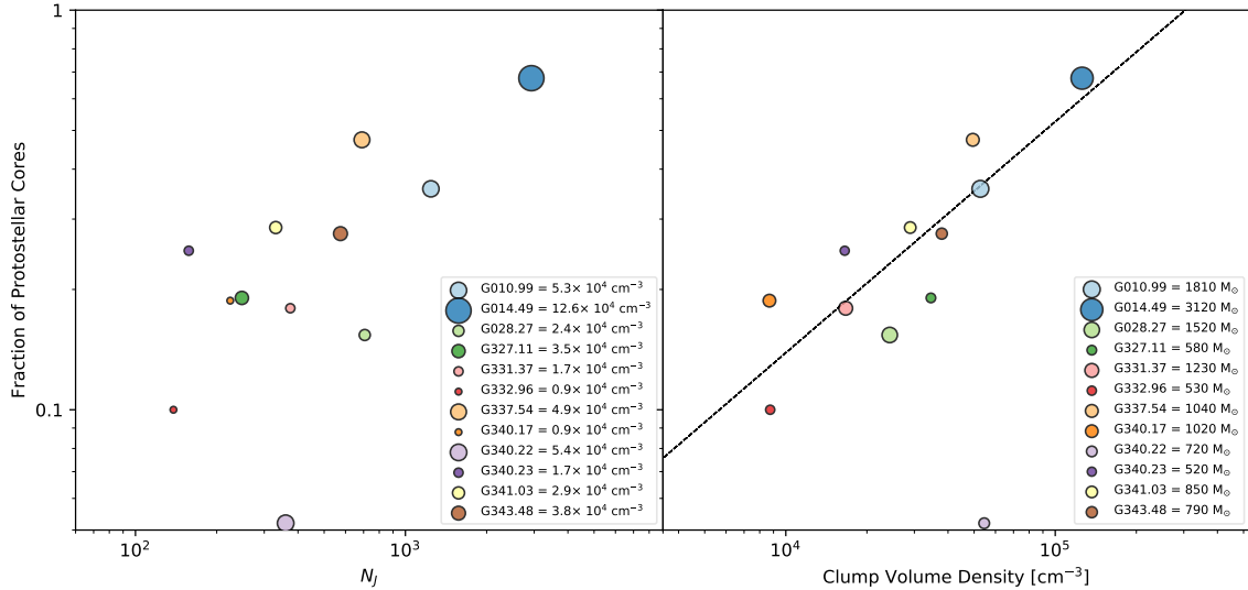
Figure 17. Left: Jeans number, N_J = M_{\text{cl}}/M_J , versus the fraction of protostellar cores per clump. A strong correlation with a Spearman correlation coefficient \rho_s = 0.52 is measured. After excluding the “outlier” clump with no protostellar cores (G340.222–00.167), the correlation becomes stronger with \rho_s = 0.6 . Right: Clump volume density against the fraction of protostellar cores per clump. The number of protostellar cores scale as \propto n_{\text{cl}}^\beta with \beta = 0.57 \pm 0.11 . For display reasons in the log-log plot, we have artificially assigned a protostellar fraction of 0.05 to G340.222–00.167.
