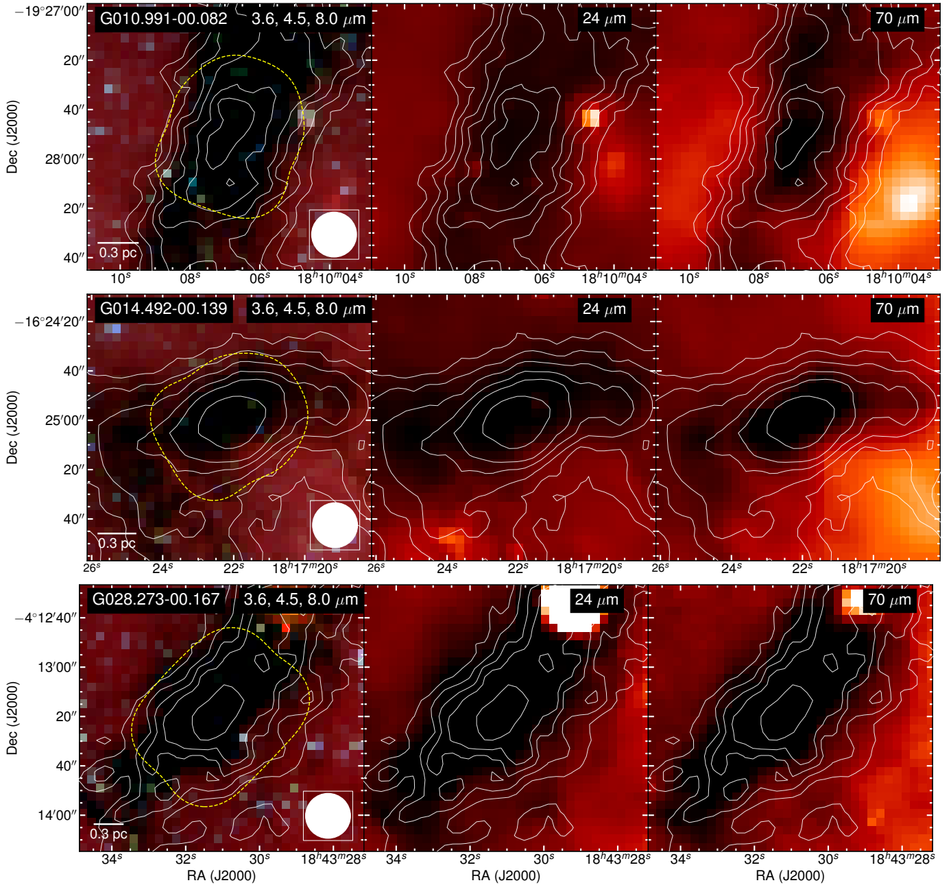
Figure 1. Spitzer and Herschel IR images for observed IRDC clumps overlaid with 870 \mu\text{m} dust continuum emission from the ATLASGAL survey (19''2; shown on the bottom right of the first panel) in white contours. Left: Spitzer /IRAC 3-color (3.6 \mu\text{m} in blue, 4.5 \mu\text{m} in green, and 8.0 \mu\text{m} in red) image. Dashed yellow contour delineates the area mosaiced with ALMA. Center: Spitzer /MIPS 24 \mu\text{m} image. Right: Herschel /PACS 70 \mu\text{m} image. Contour levels for the 870 \mu\text{m} dust continuum emission are: 3, 5, 7, 9, 12, and 15 \times \sigma , with \sigma = 71.8 \text{ mJy beam}^{-1} , for G010.991-00.082; 3, 6, 9, 13, 17, and 25 \times \sigma , with \sigma = 82.7 \text{ mJy beam}^{-1} , for G014.492-00.139; and 3, 5, 7, 9, and 12 \times \sigma , with \sigma = 64.9 \text{ mJy beam}^{-1} , for G028.273-00.167.
