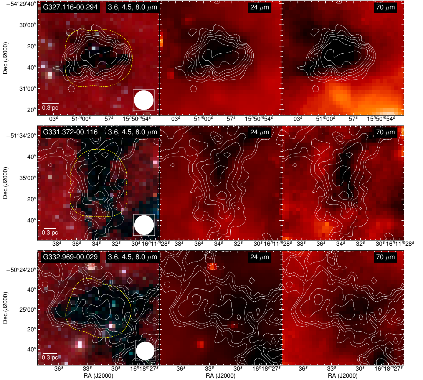
Figure 2. Same as in Figure 1, except for contour levels for the 870\ \mu\text{m} dust continuum emission, which are: 3, 4, 5, 6, 7, and 9 \times \sigma , with \sigma = 70.9\ \text{mJy beam}^{-1} , for G327.116–00.294; 3, 4, 6, 8, and 10 \times \sigma , with \sigma = 56.5\ \text{mJy beam}^{-1} , for G331.372–00.116; and 3, 4, 5, 7, and 9 \times \sigma , with \sigma = 46.9\ \text{mJy beam}^{-1} , for G332.969–00.029.
