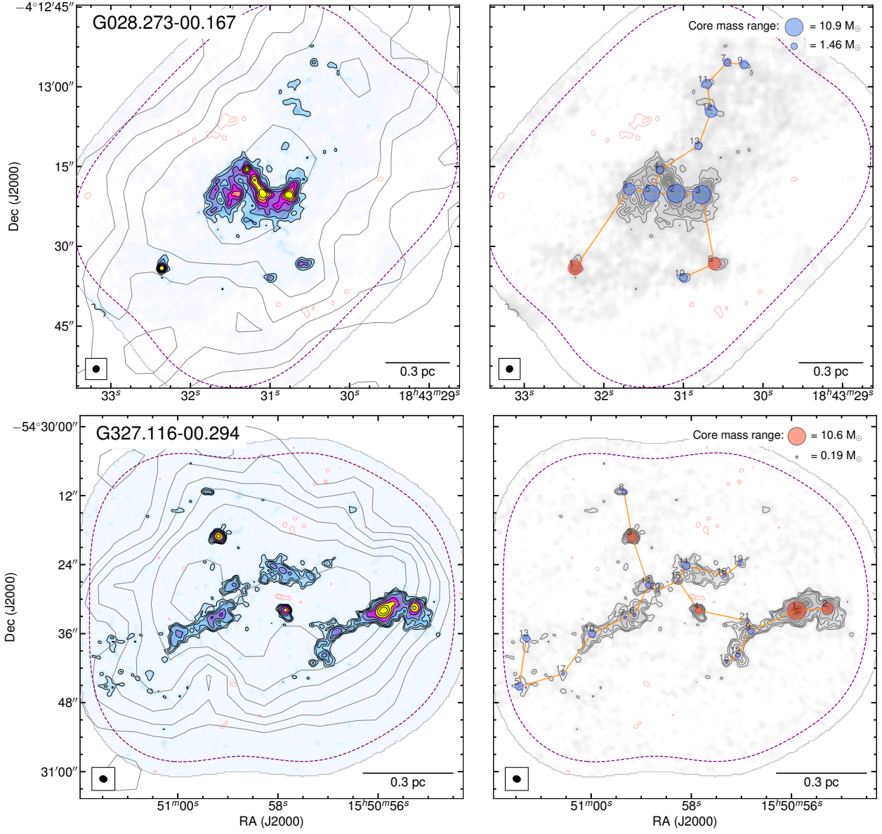
Figure 6. Same as in Figure 5, except for ALMA contour levels of -4, -3, 3, 4, 5, 6, 7, 8, and 9 \times \sigma , with \sigma = 0.164 \text{ mJy beam}^{-1} , for G028.273-00.167 ( 1''.2 angular resolution); and -4, -3, 3, 4, 5, 7, 10, 15, 23, and 35 \times \sigma , with \sigma = 0.089 \text{ mJy beam}^{-1} , for G327.116-00.294 ( 1''.2 angular resolution).
