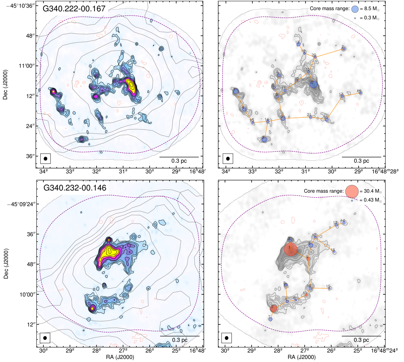
Figure 9. Same as in Figure 5, except for ALMA contour levels of -4, -3, 3, 4, 5, 6, 7, 10, 14, and 18 \times \sigma , with \sigma = 0.112 mJy beam ^{-1} , for G340.222-00.167 ( 1''.3 angular resolution); and -4, -3, 3, 4, 5, 7, 8, 11, 14, 18, and 23 \times \sigma , with \sigma = 0.139 mJy beam ^{-1} , for G340.232-00.146 ( 1''.3 angular resolution).
