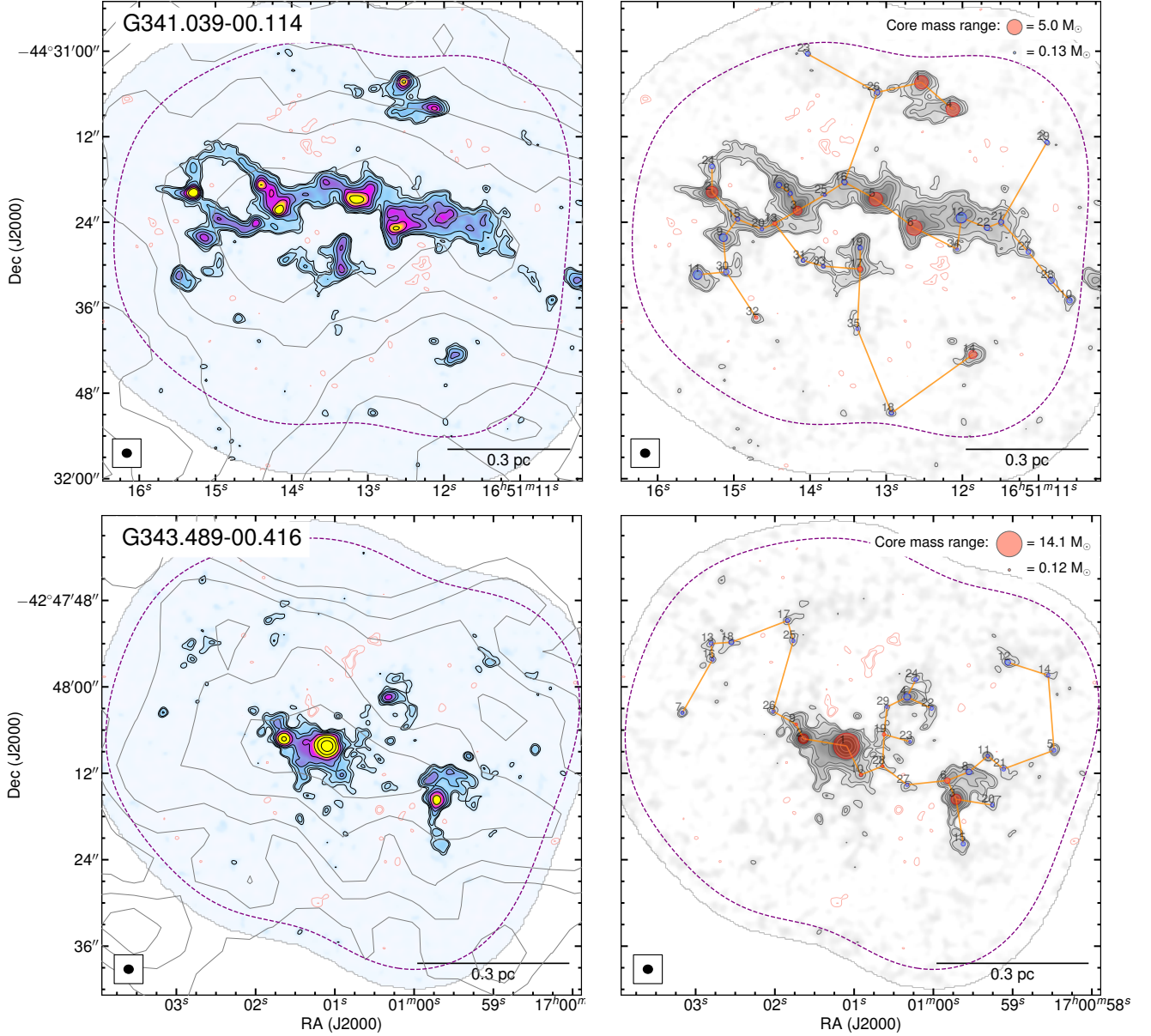
Figure 10. Same as in Figure 5, except for ALMA contour levels of -4, -3, 3, 4, 6, 9, 12, 16, and 22 \times \sigma , with \sigma = 0.070 \text{mJy beam}^{-1} , for G341.039-00.114 ( 1''.2 angular resolution); and -4, -3, 3, 4, 6, 8, 12, 20, 40, and 100 \times \sigma , with \sigma = 0.068 \text{mJy beam}^{-1} , for G343.489-00.416 ( 1''.2 angular resolution).
