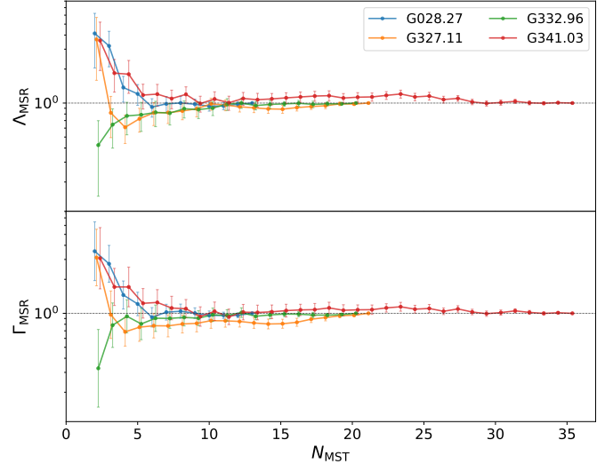
Figure 15. Mass segregation ratios ( \Lambda_{MSR} and \Gamma_{MSR} ) for different number of N_{MST} cores for the four clumps whose ratios have marginal departures from unity. For instance, if N_{MST} = 3 , \Lambda_{MSR} and \Gamma_{MSR} are calculated 1000 times from the ratio of the MST length derived from 3 random cores in the cluster and the MST length derived for the 3 most massive cores. A \Lambda_{MSR} \approx 1 (and \Gamma_{MSR} \approx 1 ) implies no mass segregation.
