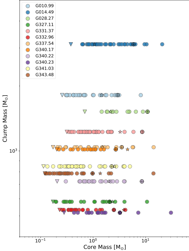
Figure 12. Clump masses against the core masses. Triangle signs indicate the 3.5\sigma level above which cores are defined. Stars signs show the value of the Jeans mass of each clump. Encircled plus signs indicate the most massive prestellar core in each clump. No correlation between the clump mass and the maximum core mass is found. A large population of low-mass cores ( < 1 M_{\odot} ) is detected. The range of core masses is well explained by thermal Jeans fragmentation, without the need of invoking turbulent Jeans fragmentation.
