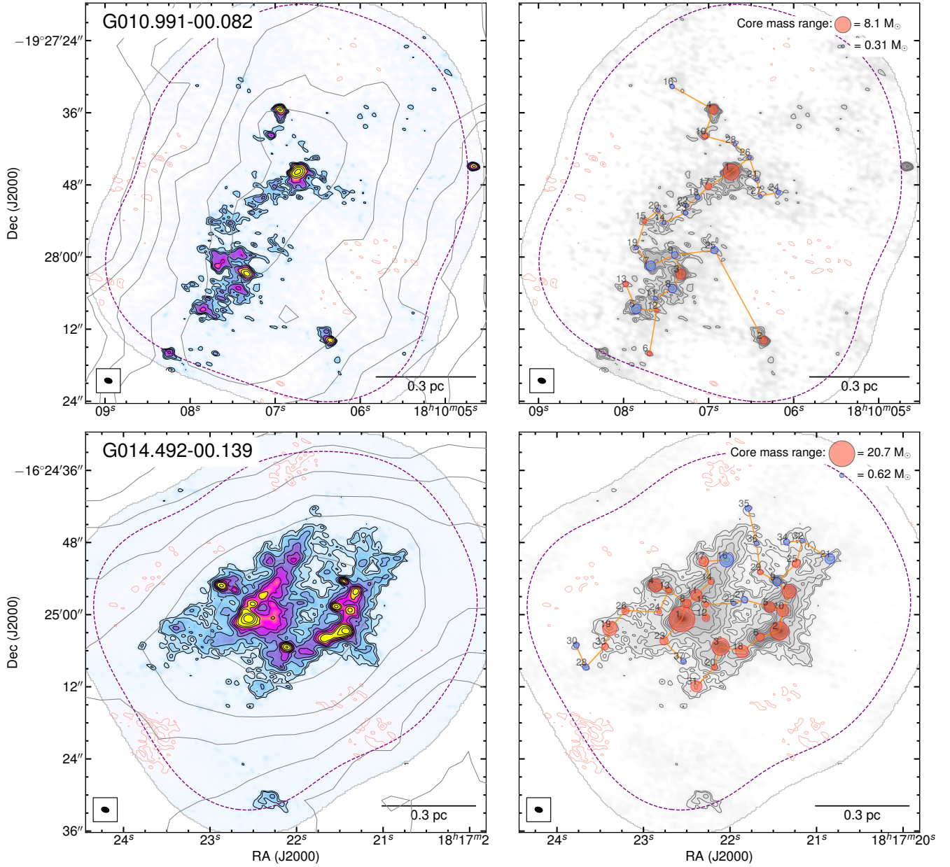
Figure 5. ALMA 1.34 mm dust continuum emission for two IRDC clumps. Dashed purple contour delineates the area mosaiced with ALMA. Left: color image and small-scale contours correspond to the ALMA dust continuum emission (12 and 7 m array combined). ALMA contour levels are -4, -3, 3, 4, 5, 7, 10, 14, and 20 \times \sigma , with \sigma = 0.115 \text{ mJy beam}^{-1} , for G010.991-00.082 ( 1''.1 angular resolution); and -4, -3, 3, 4, 6, 8, 10, 12, 15, 18, 25, and 35 \times \sigma , with \sigma = 0.168 \text{ mJy beam}^{-1} , for G014.492-00.139 ( 1''.1 angular resolution). Grey and red contours mark the positive and negative levels, respectively. Synthesized beams are displayed at the bottom left in each panel. Large-scale contours delineate the single-dish dust continuum emission from ATLASGAL (contour levels are the same as in the corresponding Figure 1, 2, 3, or 4). Right: gray-scale image and contours correspond to the ALMA dust continuum emission (12 and 7 m array combined). Blue circles show the positions of the prestellar core candidates, while the red circles show the positions of the protostellar cores (see Section 4.3). The circle size is proportional to the core mass and the range of mass values is displayed on the top, right side of the panel. Numbers near each core correspond to the core name (ALMA1, ALMA2, ...), where the prefix ALMA has been dropped for clarity. Orange segments show the outcome from the minimum spanning tree (MST; Section 5.4.1), which corresponds to the set of straight lines that connects cores in a way that minimize the sum of the lengths.
