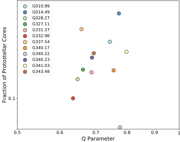
Figure 14. Spatial distribution of cores (characterized by the Q parameter) versus the fraction of protostellar cores per clump, as a proxy of clump evolution. A weak correlation with a Spearman correlation coefficient \rho_s = 0.28 is measured. After excluding the “outlier” clump with no protostellar cores (G340.222–00.167), the correlation becomes stronger with \rho_s = 0.59 . For display reasons in the log-log plot, we have artificially assigned a protostellar fraction of 0.05 to G340.222–00.167.
