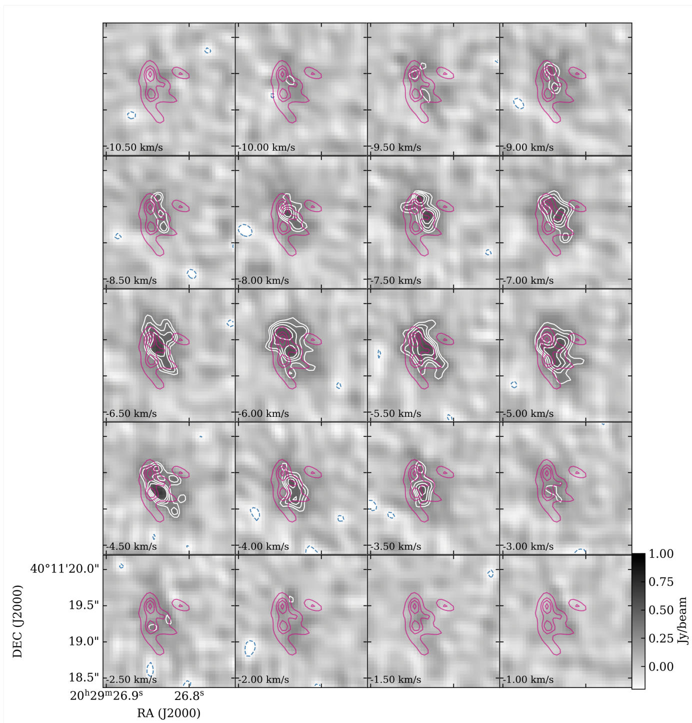
Fig. A.1. Channel maps of HCN v_2=1 emission with the emission levels of 5, 6, 7, and 8 \sigma are marked with white contours. The magenta contours mark the 3, 5, 6, and 7 \sigma 843 \mu\text{m} continuum emission. The blue dashed contours indicate the -3\sigma line emission.
