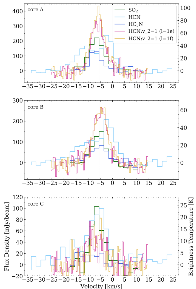
Fig. 3. Spectra of the five most prominent transitions towards the center of the cores A (top panel), B (middle panel), and C (bottom panel) averaged over a beam size. The vertical gray dashed line indicates the source velocity.
