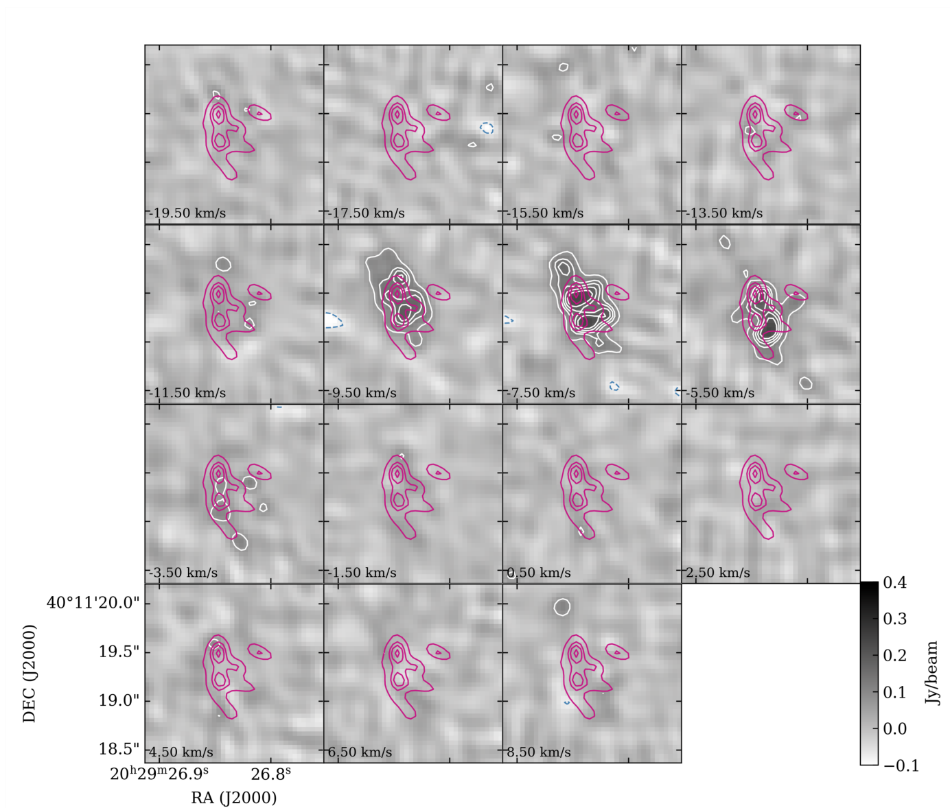
Fig. A.5. Channel maps of \text{HC}_3\text{N} emission with the emission levels of 3 , 5 , 6 , and 7\sigma are marked with white contours. The magenta contours mark the 3 , 5 , 6 , and 7\sigma 843\ \mu\text{m} continuum emission. The blue dashed contours indicate the -3\sigma line emission.
