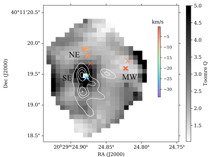
Fig. 6. Toomre Q map taken from Ahmadi et al. in prep. overlaid with the 843 \mu\text{m} continuum contours in white (3, 5, 6, and 7\sigma ) and the water maser locations from Sanna et al. (2012). The water masers are shown with colored crosses where the color represents their radial velocity and for their locations, we use the same naming convention northeast (NE), southeast (SE), and middle-west (MW) as Sanna et al. (2012). The blanked pixel in the Toomre Q map near core A is the assumed location of the protostar.
