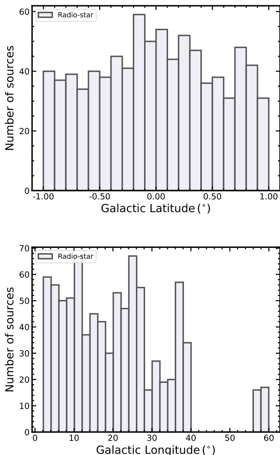
Fig. 19. Distribution of radio star candidates as a function of Galactic Latitude (upper panel) and Longitude (lower panel) for the GLOSTAR B-configuration catalog, including the catalog of this work ( 2^\circ < \ell < 28^\circ , 36^\circ < \ell < 40^\circ & 56^\circ < \ell < 60^\circ and |b| < 1^\circ ), as listed in Table 3 and the published pilot catalog ( 28^\circ < \ell < 36^\circ and |b| < 1^\circ ) in Table 1 of Dzib et al. (2023). The bin sizes are 0.1^\circ and 2.0^\circ for the upper and lower panel, respectively. The blank region in Galactic longitude 40^\circ < \ell < 56^\circ is not covered by the GLOSTAR survey in B-configuration.
