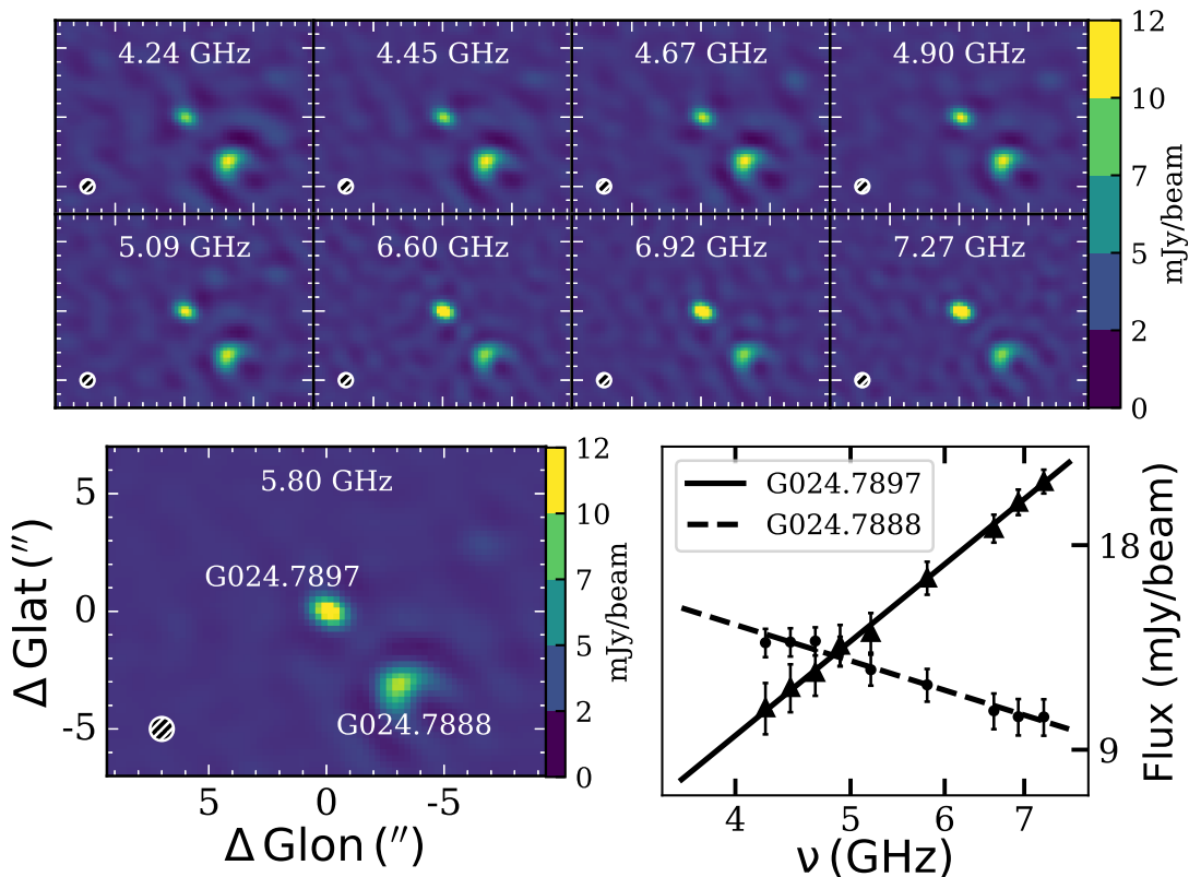
Fig. 18. The example of two H II region candidates with positive and negative in-band spectral index, as discussed in Sect. 5.2. The top two rows show the 8 sub-bands of the GLOSTAR image. The bottom-left panel shows the averaged image at 5.8 GHz used to extract the source, and the bottom-right panel shows the in-band spectral index fitting for the two compact H II regions candidates: the solid line for G024.7897 ( Y_{\text{factor}} = 1.02 ) with \alpha = 1.43 \pm 0.02 and the dashed line for G024.7888 ( Y_{\text{factor}} = 1.97 ) with \alpha = -0.55 \pm 0.04 . The FWHM beam of GLOSTAR in B-configuration (1.0'') is indicated by the white circles in the lower-left corner of each image. There is a clear trend that the fluxes increase and decrease as the increasing frequencies in the sub-bands for G024.7897 and G024.7888 respectively.
