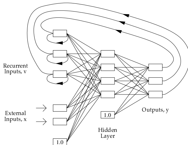
Fig. 6: A recurrent neural network architecture (‘dynet’) for modelling dynamical systems. The outputs, \mathbf{y} , from the network are the time derivatives of the state variables of the dynamical system. The recurrent inputs, \mathbf{v} , are these state variables. The values of \mathbf{v} at the next time step are evaluated (using equation 9) from the outputs (via the recurrent connections) and the previous values of \mathbf{v} . All connections and the two bias nodes are shown.
