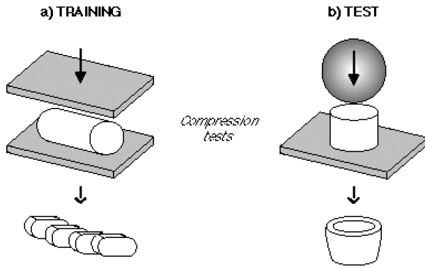
Fig. 1: Deformation geometries. (a) Plane-strain diametrical compression. The workpiece is subsequently sectioned into many nominally identical specimens which are annealed at different combinations of temperature and time. The compression gives rise to a non-linear distribution of strains across the specimen (see Figure 2b). These allow us to obtain many input training vectors, \mathbf{x} , for our model using a single compression test. (b) Axisymmetric axial compression.
