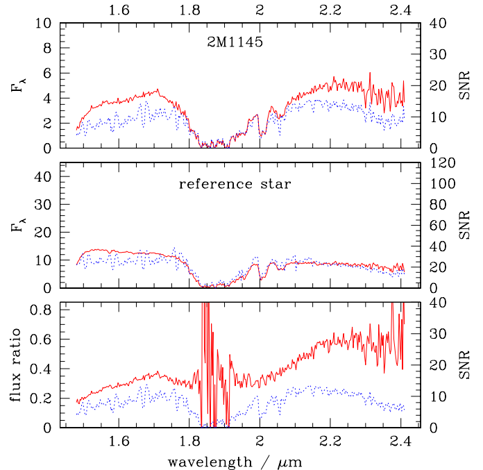
Fig. 7. Same as Fig. 6 but for the HK filter. The spectra are from the fifth sequence on night 1. The flux is in the same (arbitrary) units as in Fig. 6. The low signal and SNR between 1.80 and 1.95 \mu\text{m} is due to strong water absorption by the Earth’s atmosphere.
